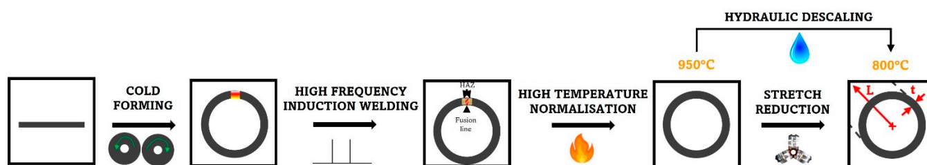
Figure 1. Schematic sequence of the conveyance tube manufacturing process.
