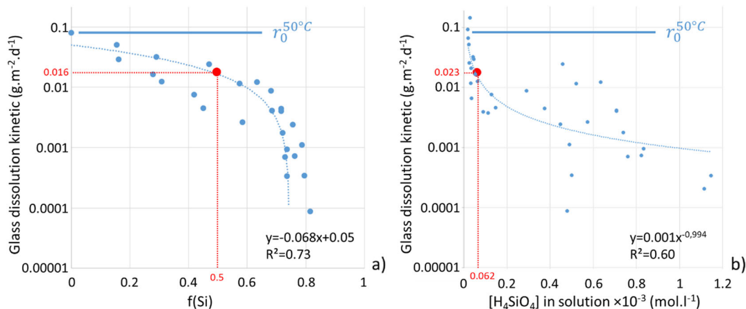
Fig. 8 Estimated glass dissolution kinetics in function of silicon retention ( f(\text{Si}) ) or \text{H}_4\text{SiO}_4 concentration in solution. According to the f(\text{Si}) = 0.5 in GAL and the [\text{H}_4\text{SiO}_4] = 0.062 \text{ mol l}^{-1} in solution, the glass alteration rates associated with these values are respectively 1.6 \times 10^{-2} \text{ g m}^{-2} \text{ j}^{-1} (a) and 2.3 \times 10^{-2} \text{ g m}^{-2} \text{ j}^{-1} (b).
