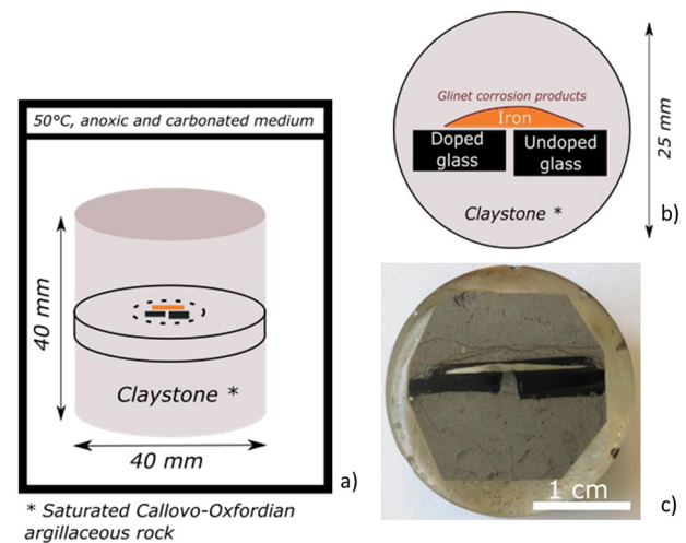
Fig. 1 Experimental setup of the glass/iron/claystone system. Arrangement of the two SON68 glass coupons pressed against a piece of iron in the Cox claystone cylinder (a), and cross section obtained on the system (b and c).
