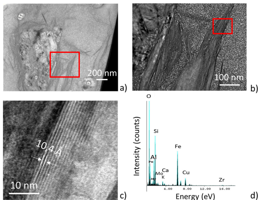
Fig. 4 TEM analyses in the o-GAL. High resolution TEM micrographs (a + b + c) highlighting the presence of crystalline phases with inter-reticular distance of 10.4 Å ( \sigma = 0.6 ) compatible with smectite group. TEM-EDS spectrum (d) corresponding to the crystalline phase (composition in Table 2).
