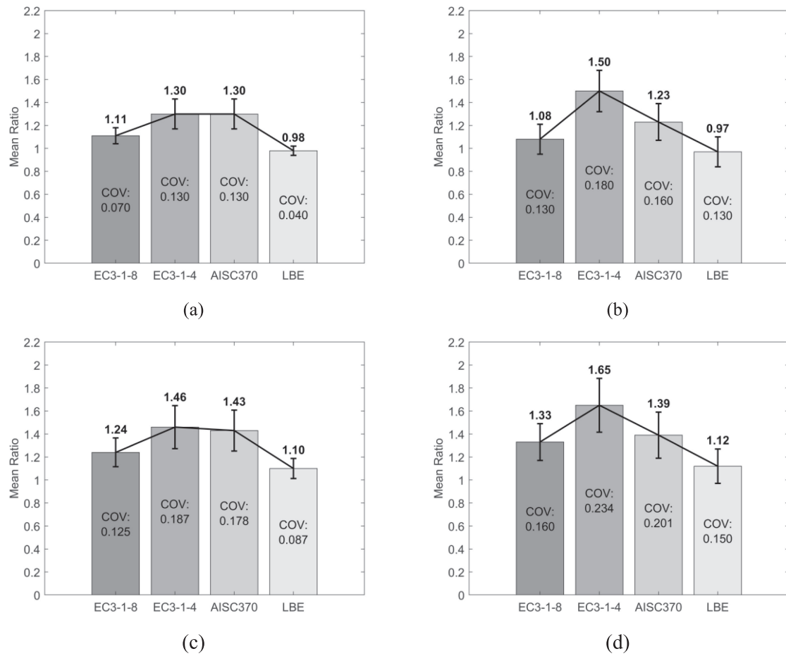
FIGURE 7 | Comparison of design provisions [12, 13, 20] and LBE [5, 22] estimations against experimental load capacity plates: mean ratios and COV of CON plates in (a) single-bolt and (b) double-bolt configurations and for AM plates in (c) single-bolt and (d) double-bolt configurations.
