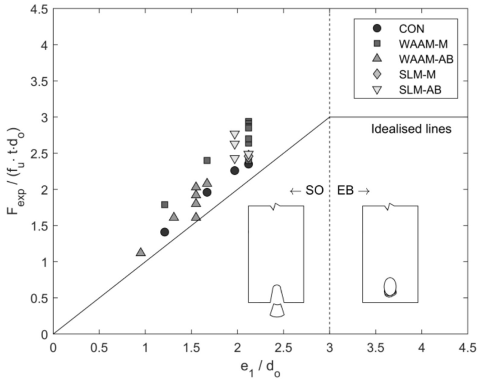
FIGURE 8 | Indirect interpretation of EC3-1-8 [12] showing the threshold between EB and SO governing failures for single-bolted configurations connection results, using the condition e_1 / d_o < 3 as derived from the definition of a_b in [5].
