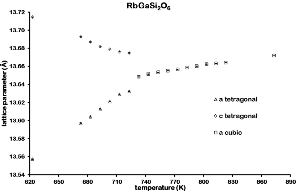
Figure 5. Variation of lattice parameters for RbGaSi 2 O 6 from 623 to 873 K.
