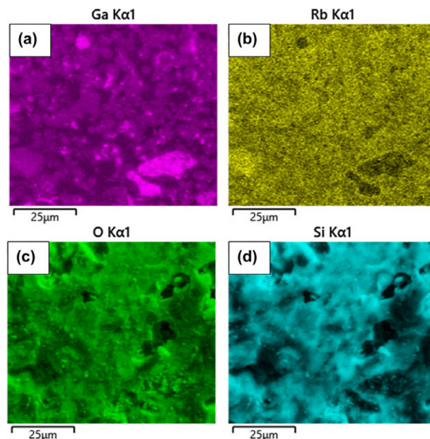
Figure 9. Qualitative EDX mapping of the \text{RbGaSi}_2\text{O}_6 sample: (a) gallium map; (b) rubidium map; (c) oxygen map; and (d) silicon map.
