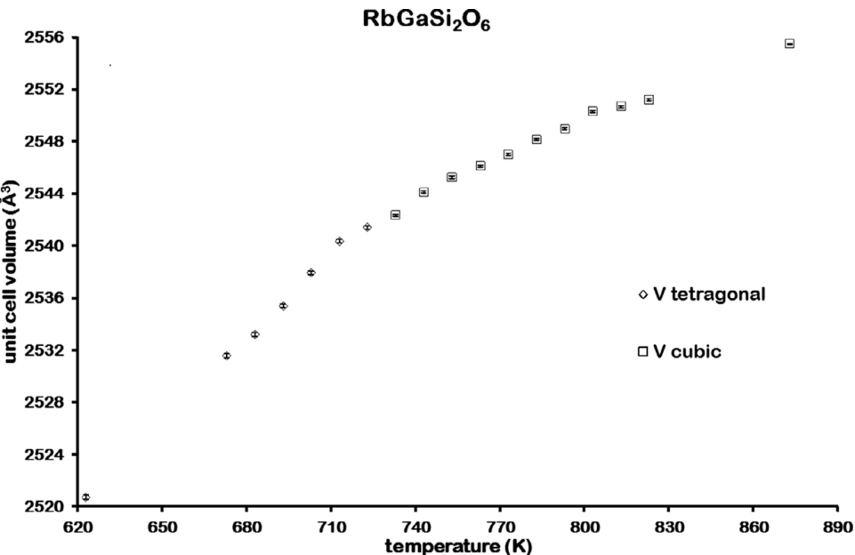
Figure 6. Variation of unit cell volume for RbGaSi 2 O 6 from 623 to 873 K.
