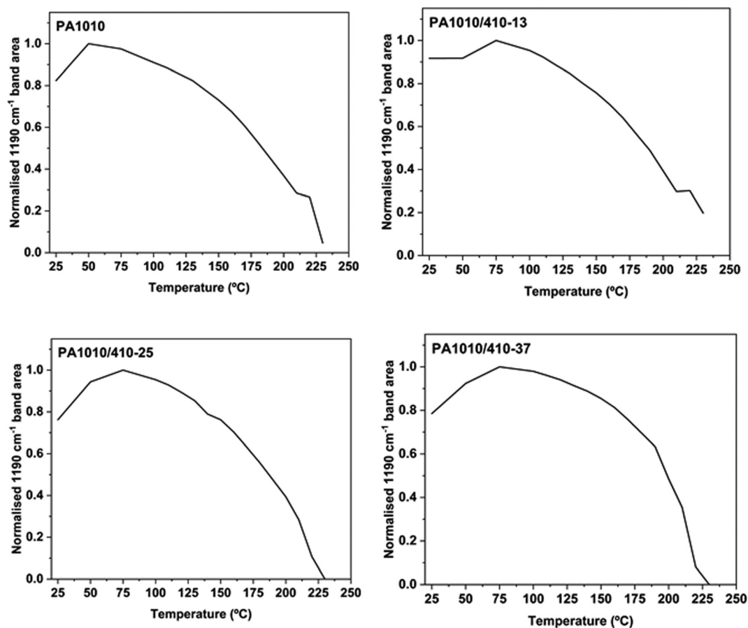
Fig. 10 Normalized area corresponding to 1190 cm -1 band of polyamide 1010 (PA1010) and copolyamides 410/1010: PA1010/410 with 12.5, 25 and 37.5 mol% nylon 410.
