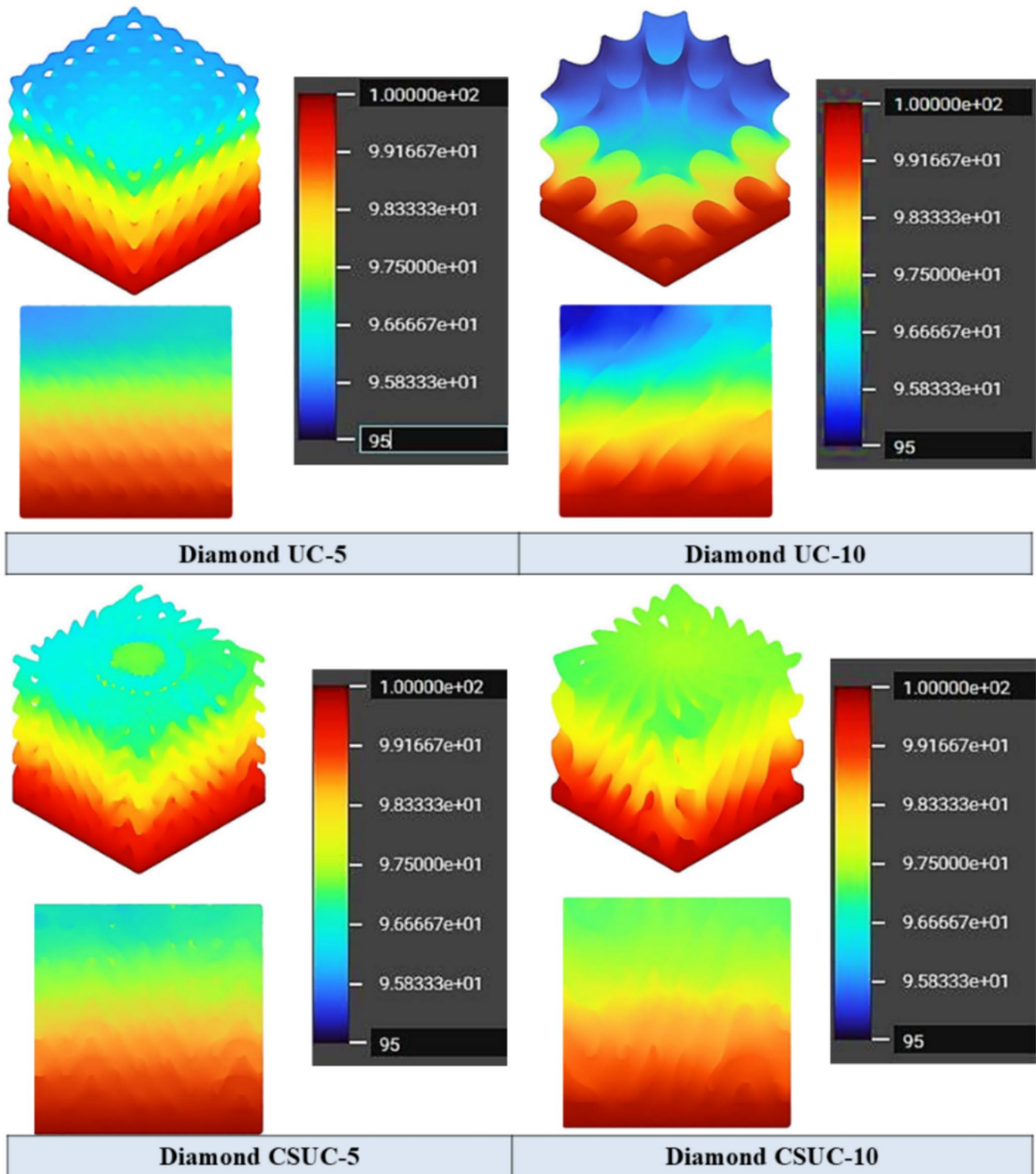
Fig. 7 Temperature contours for the diamond heat sinks (3D and front view)
