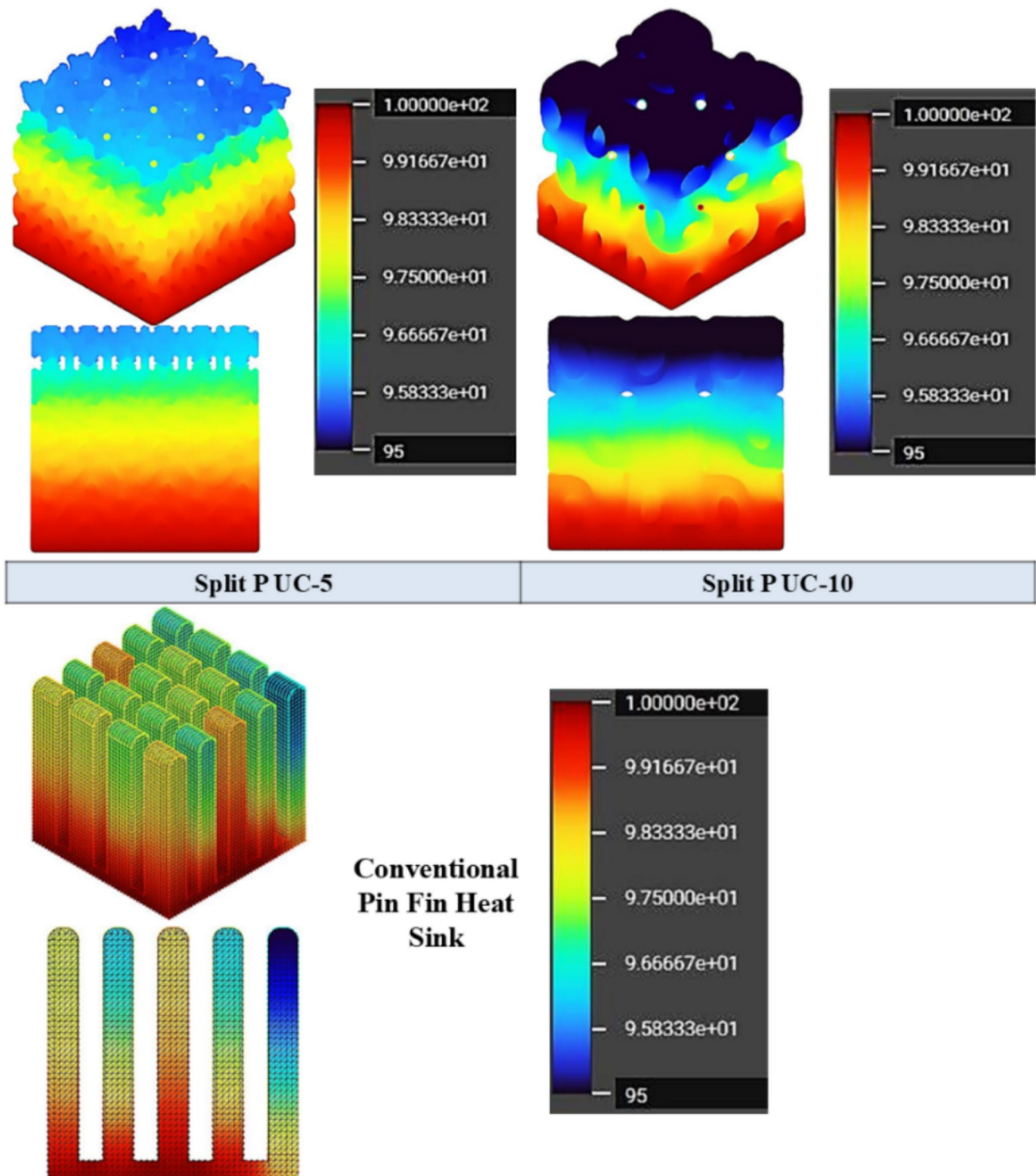
Fig. 10 Temperature contours for split-p and conventional pin fin heat sinks (3D and front view)
