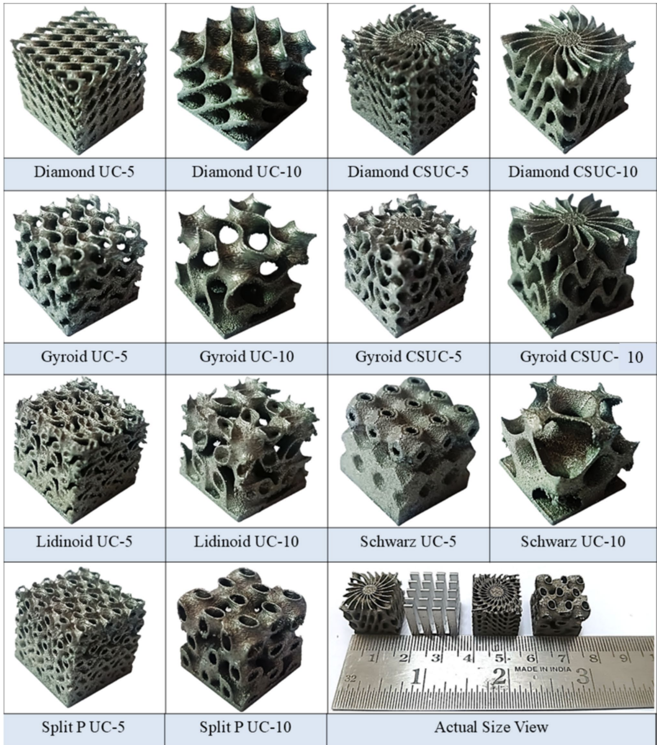
Fig. 5 A20X metal lattice heat sinks with varying unit cell sizes fabricated using LPBF
