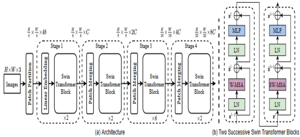
Figure 1. Swin Transformer architecture with equation [29].
