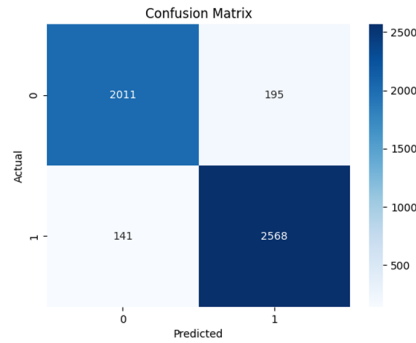
Figure 10. Confusion matrix of ViT-Base.
