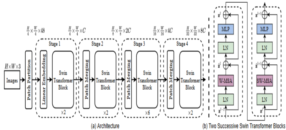
Figure 1. Swin Transformer architecture with equation [29].
