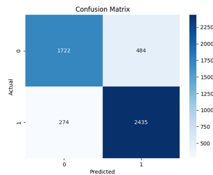
Figure 9. Confusion matrix of ResNet50.
