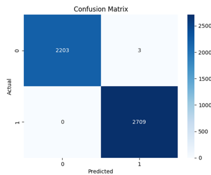
Figure 11. Confusion matrix of Swin Transformer.
