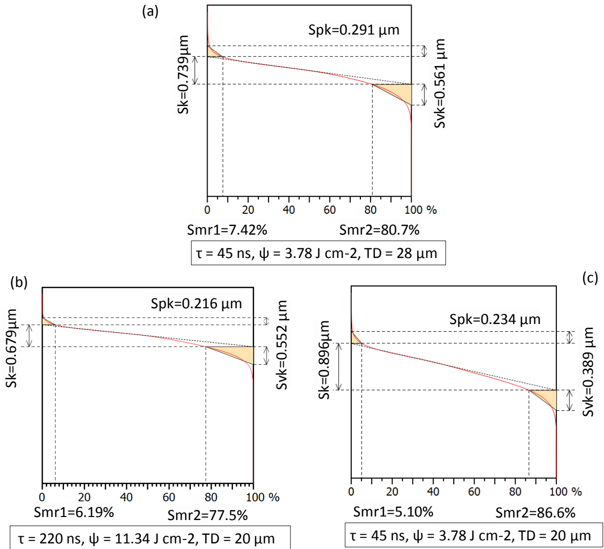
Figure 15: Abbott curve for a single profile and the parameters Sk , Spk and Svk of CTM302 milled at I 100%, FS 1000 \text{mms}^{-1} .
