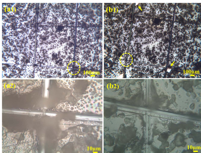
Fig. 10 Crosshatch test (a1) and (a2) encircled areas are before the adhesive tape was applied (b1) and (b2) after the tape was applied.
