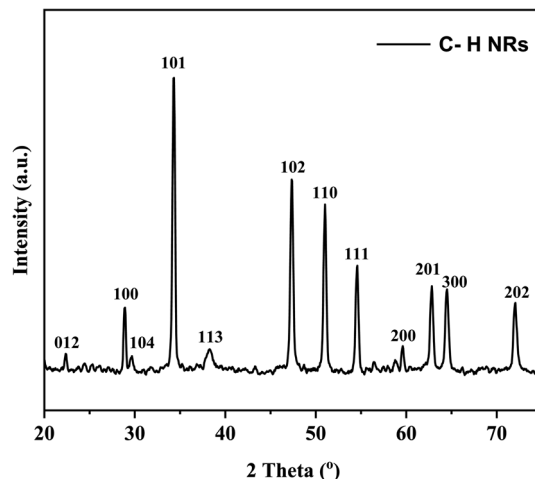
Fig. 3 X-ray diffraction of C-H NRs.
