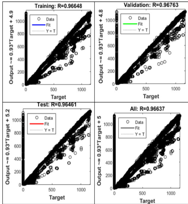
FIGURE 7. The performance of the Levenberg-Marquardt on NARX.
