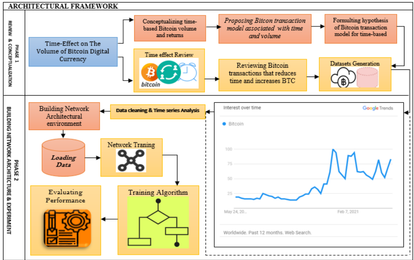
FIGURE 1. Architectural framework.
