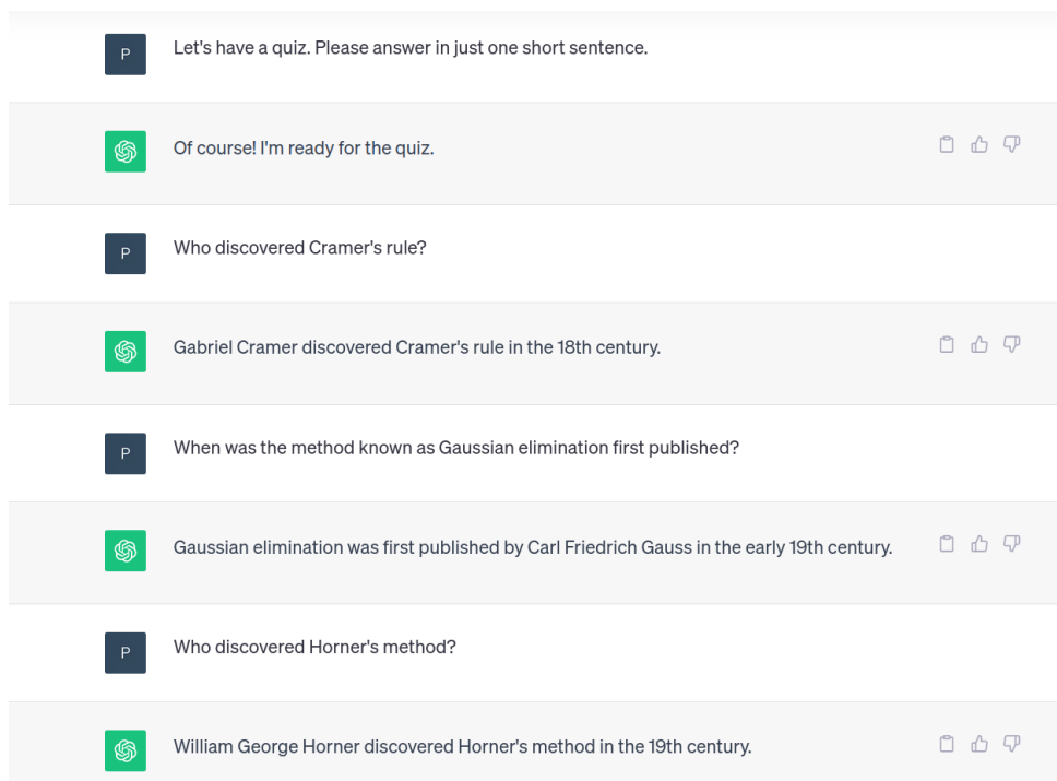
Figure 1: ChatGPT interface showing responses to prompts given.
