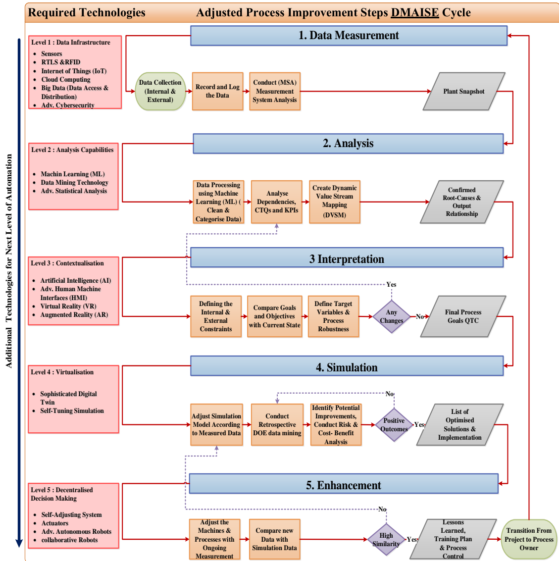
Figure 7. Illustrates the contents of the DMAISE cycle, including its phases, required technologies, processes and output of each phase.
