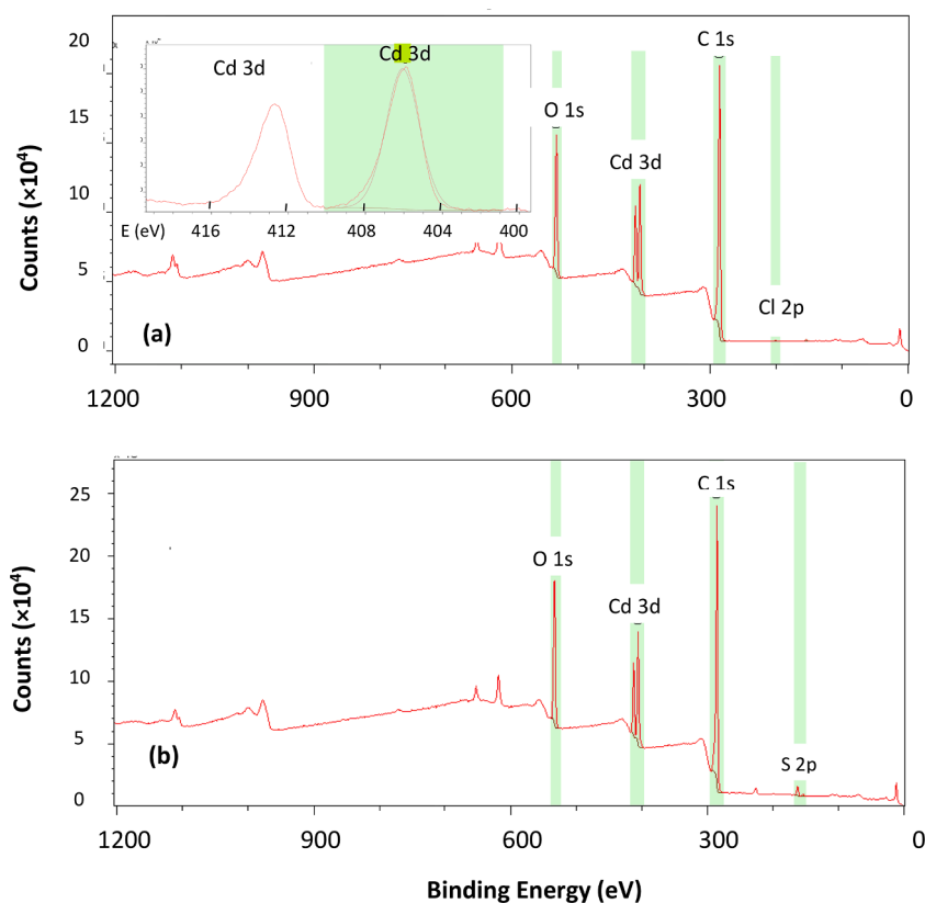
Fig. 6. Typical XPS scans for LB films (40 layers) containing Cd before (a) and after (b) treatment with H 2 S. Inset shows Cd 3d peaks zoomed in.
