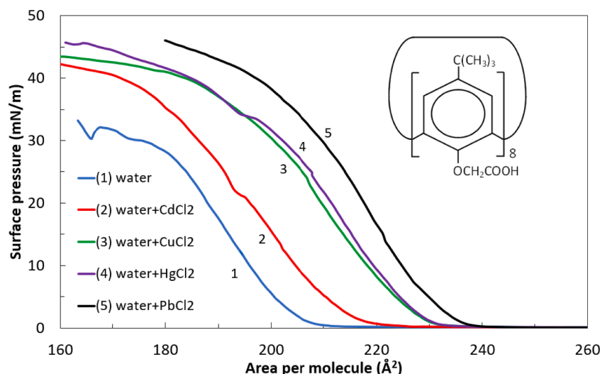
Fig. 1. Surface pressure -area isotherms of the calix(8)arene on water (1) and subphases containing 0.5 mM metal chlorides (2–5). Inset shows the chemical structure of octa-tertbutyl-calix(8)arene carboxylic acid.
