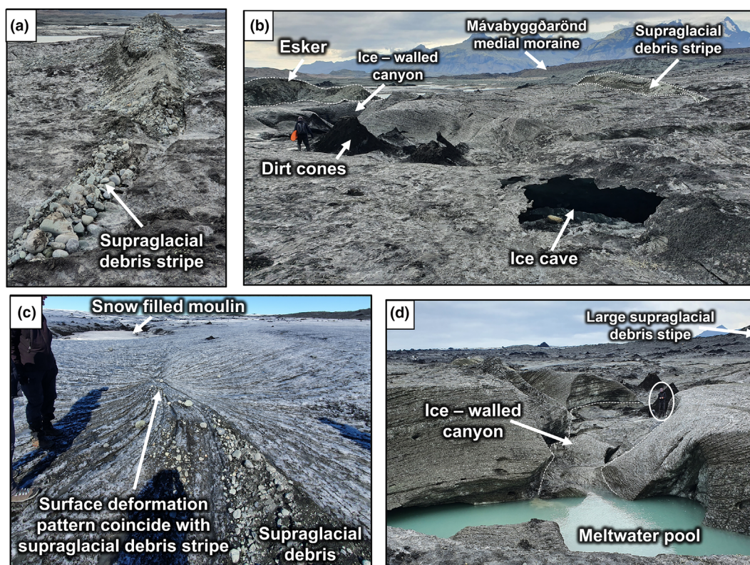
FIGURE 9 Selection of field photos: (a) supraglacial debris melting out of the ice (photo facing west); (b) the large moulin area in September 2022, the moulin has evolved into an ice-walled canyon; (c) deformation patterns on the surface of the ice. They appear to spread from a point which coincides with a supraglacial debris stripe. The May 2022 slow filled moulin is visible upglacier (photo facing north); (d) view upglacier of the previous moulin area which is now an ice-walled channel with meltwater pooling northeast of the September 2022 esker, circled person 1.8 m for scale (photo facing northeast). [Color figure can be viewed at wileyonlinelibrary.com ]
