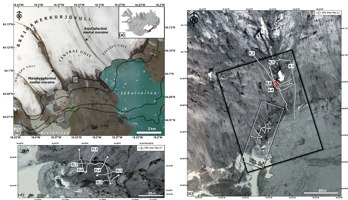
FIGURE 1 (a) Copernicus EU-DEM of Iceland and Vatnajökull ice cap with Breiðamerkjökull marked by the red dot; (b) Breiðamerkjökull and associated foreland (Sentinel-2 harmonised true colour image from 6 May 2022) with extent of Figure 1c (white box) shown. The central unit (Esjufjallajökull) is delineated by two medial moraines: Mávabyggðarönd to the west and Esjufjallarönd to the east. Several terminus locations are noted from 1985 to present; (c) GPR survey lines collected in May 2022, overlain on the May 2022 orthomosaic generated from UAV data. The arrows indicate the acquisition direction. On-ice GPR lines shown in Figure 8 are labelled IL1-5. Extents for Figures 1d and 3 are shown; (d) Zoomed-in view of esker cross and crestline (Figure 7, EL1-6) GPR profiles, overlain on the May 2022 orthomosaic. [Color figure can be viewed at wileyonlinelibrary.com ]
