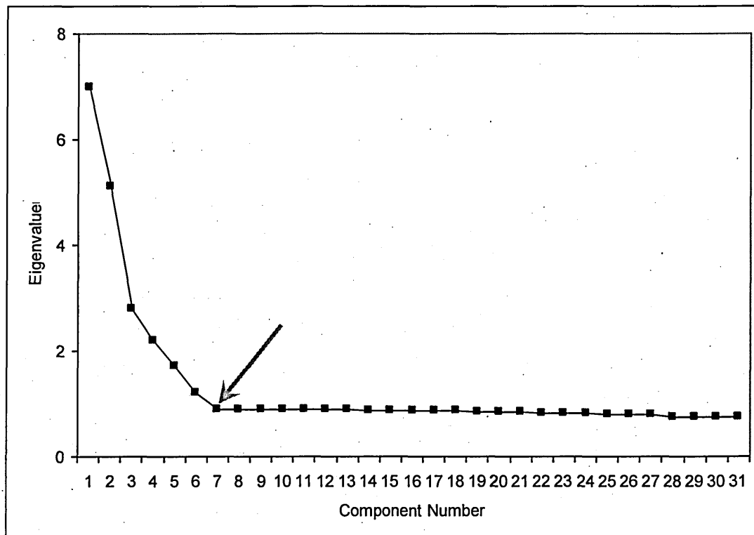
Figure 6.3: Scree plot test – seven dimensions
