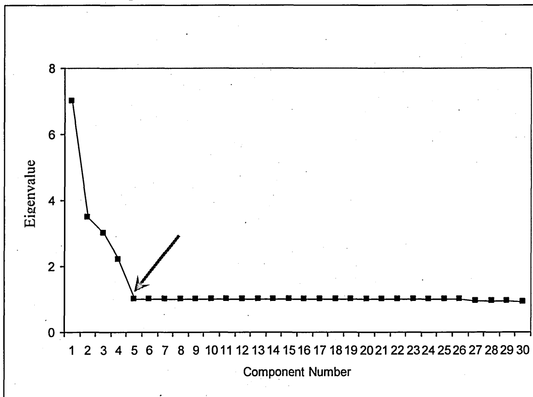
Figure 7.3: Scree plot test – Five dimensions.
