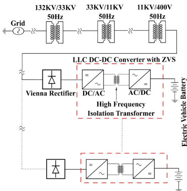
Figure 2. EV charging system from 400V AC mains
