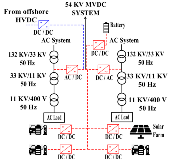
Figure 1. Proposed MVDC Transmission in red
