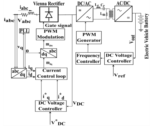
Figure 5. Converter control system implemented in Simulink
