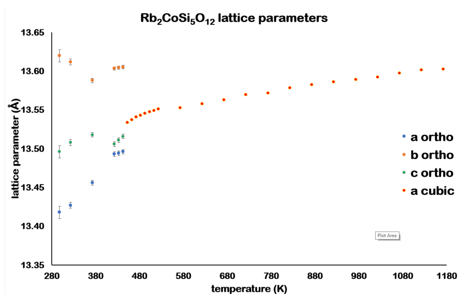
Figure 7. Variation of Pbca orthorhombic a , b and c lattice parameters and Pa\bar{3} cubic a lattice parameter with calibrated temperatures for \text{Rb}_2\text{CoSi}_5\text{O}_{12} .
