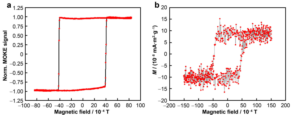
Fig. 2 Magnetic hysteresis loops of glass/Ta (5 nm)/Pt (2 nm)/Co (0.6 nm)/Pt (2 nm) sample at room temperature: a measured by MOKE image system; b measured by VSM
