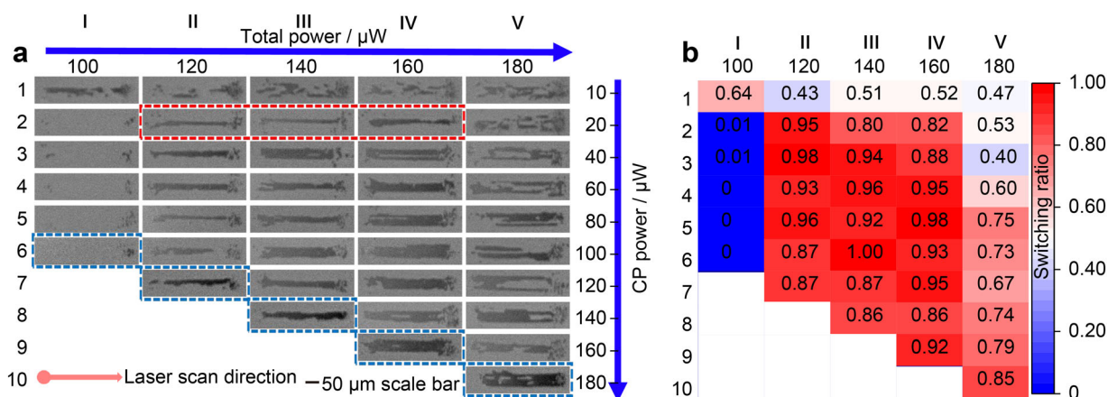
Fig. 4 HD-AOS induced by dual-pump with different power combinations at a fixed time interval: a MOKE images of magnetic domains induced by a sequence of LP and CP pulse pairs; b extracted switching ratio for each image frame
