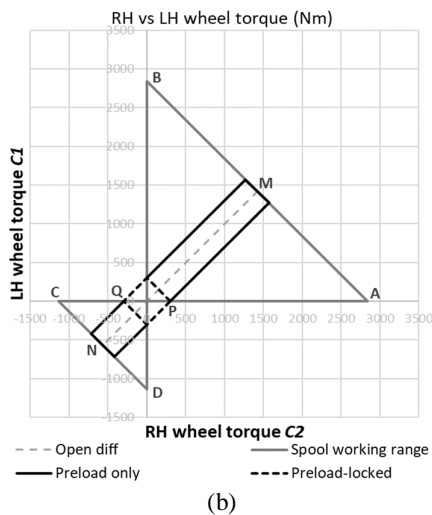
Figure 13. Torque bias diagrams for preload only. Preload value = 300 Nm.
