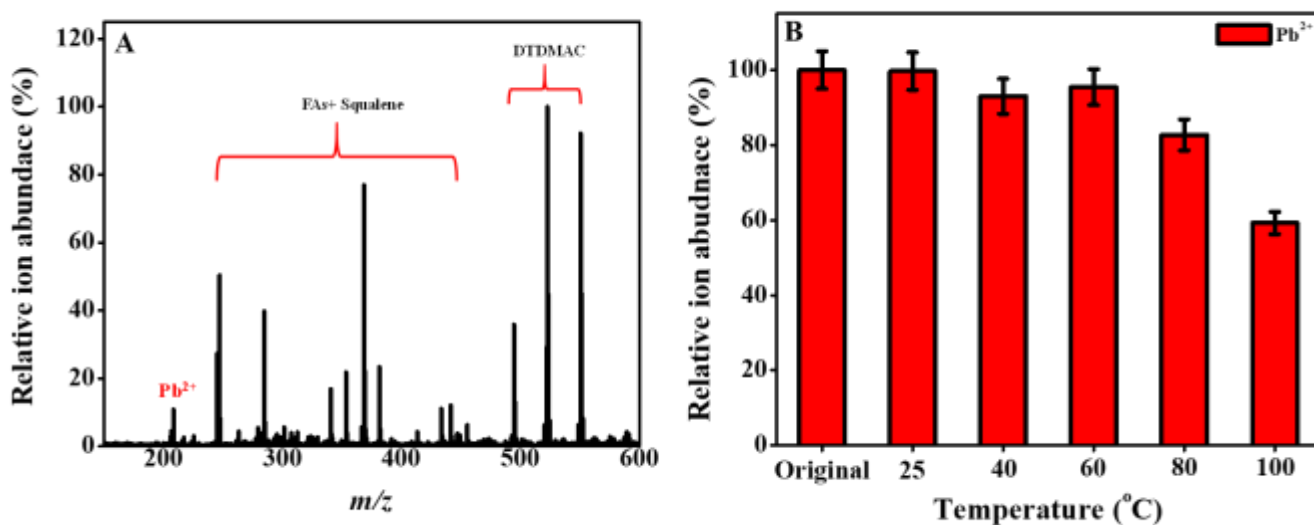
Figure 3: Detection of lead in contaminated fingermark A) SALDI-MS spectrum of fingermark contaminated with lead and B) effect of temperature on the analysis of lead contaminated fingermark. Error bars represent standard deviation for five replicates.
