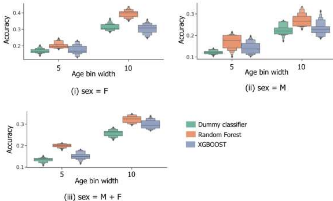
Fig. 4. Distribution of categorical age prediction scores across XGBOOST, random forest and baseline dummy classification model types, for models trained on (i) female sample data only, (ii) male sample data only, (iii) the combined sample set of male and female data. Age is expressed in years.
