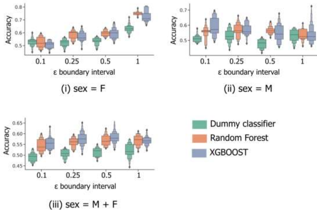
Fig. 3. 5-fold cross validation performance results for binary classification models predicting binary old/young donor labels for XGBOOST, random forest and baseline dummy classification model types. Performance statistics are presented separately for models trained using (i) female-only, (ii) male-only data, in addition to (iii) the full sample set. Each x-axis illustrates the effect of \epsilon , the parameter dictating the size of the masked sample region between the “young” and “old” age classes, (\mu_{age} - \epsilon \cdot \sigma_{age}, \mu_{age} + \epsilon \cdot \sigma_{age}) . Each boxplot summarises the distribution in accuracy scores across all 4 feature selection strategies and peak picking strategies from Heaton et al. , 6 .
