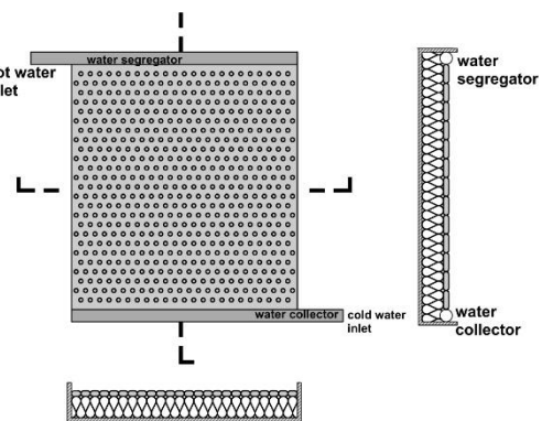
Figure 13: Ceiling night radiator (Man et al., 2015)
