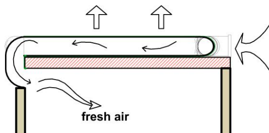
Figure 10: Radiator model (Bagiorgas and Mihalakou, 2008)
