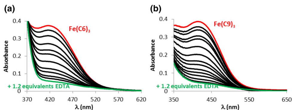
Fig. 3 Spectrophotometric batch competition titration between a Fe(C6) 3 ([C6] = 3.65 \times 10^{-4} M, [C6]/[Fe 3+ ] = 3.2) and EDTA ( 0 \leq [\text{EDTA}]/[\text{Fe(C6)}_3] \leq 1.2 ), and b Fe(C9) 3 ([C9] = 3.54 \times 10^{-4} M, [C9]/[Fe 3+ ] = 3.2) and EDTA ( 0 \leq [\text{EDTA}]/[\text{Fe(C9)}_3] \leq 1.2 ). Solvent: Hepes buffer pH 7.4, I = 0.1 M (NaClO 4 ), T = 25.0 °C
