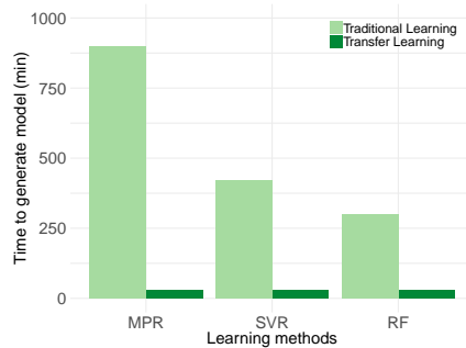
Fig. 13. The time taken to generate models using traditional ML and TL.
