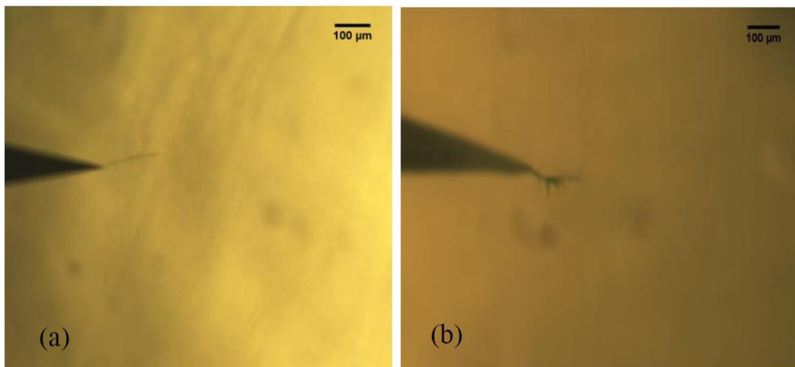
Figure 4. Development of electrical treeing (ETs) at direct current (DC) voltage (a) +28 kV and (b) −28 kV [23].
