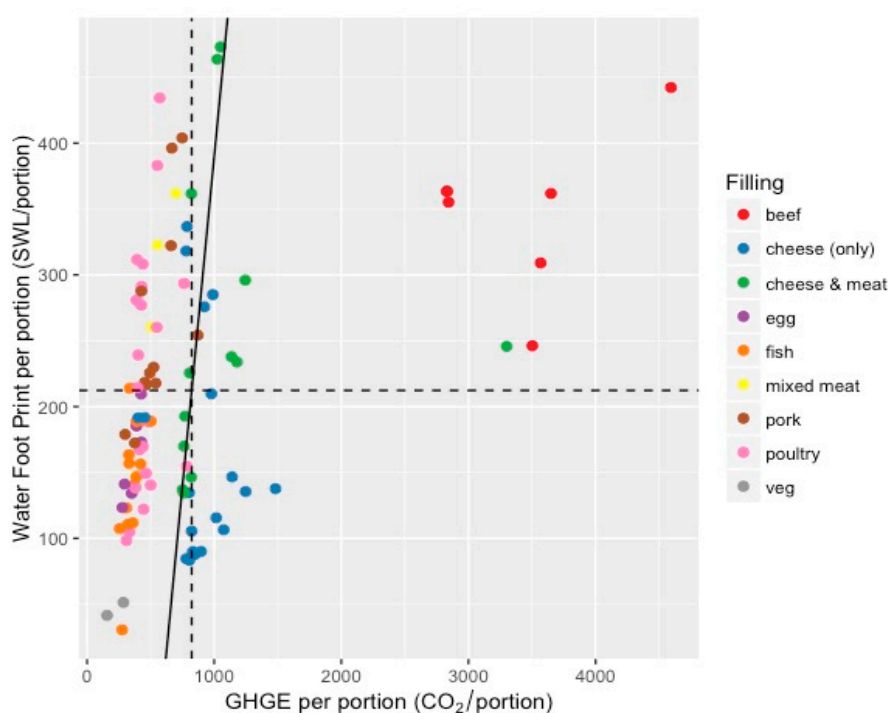
(a) Environmental impact score of sandwiches (n = 101)
