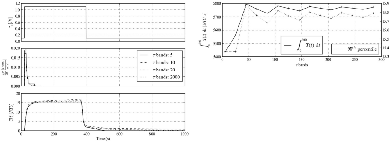
(a) dN(t)/dt and T(t) for a constant \tau range but different values of \Delta\tau (given a pulse increase in \tau_a ).
