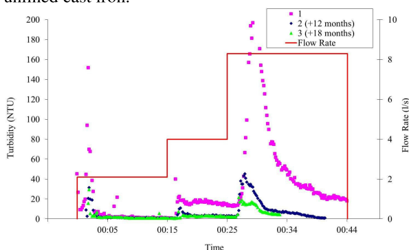
(c) Surface water / groundwater blend, ID=72mm, polyethylene.
