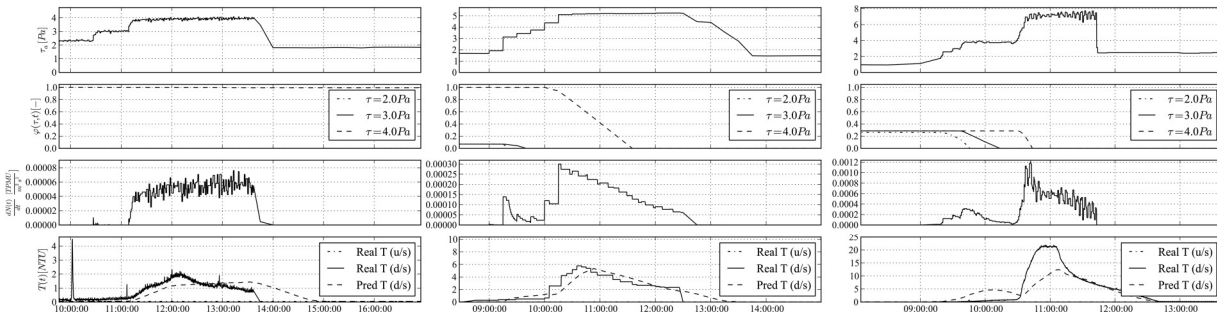
Figure 5: Model validation for 3.7km-long trunk main. (a) Boundary shear stress profile, (b) predicted variation in relative material quantity \varphi for selected shear strength bands, (c) predicted material flux rate dN(t)/dt from each m^2 of pipe wall and (d) predicted and observed turbidity response at the downstream ('d/s') end of the main for each of three successive flow trials.
