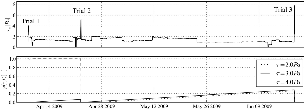
Figure 4: Details of model validation for 3.7km-long trunk main. (a) Boundary shear stress profile over and between three flow trials covering a 72.2 day period; (b) The variation in relative material quantity \varphi for three selected shear strength bands shows erosion and regeneration occurring at different strengths.
