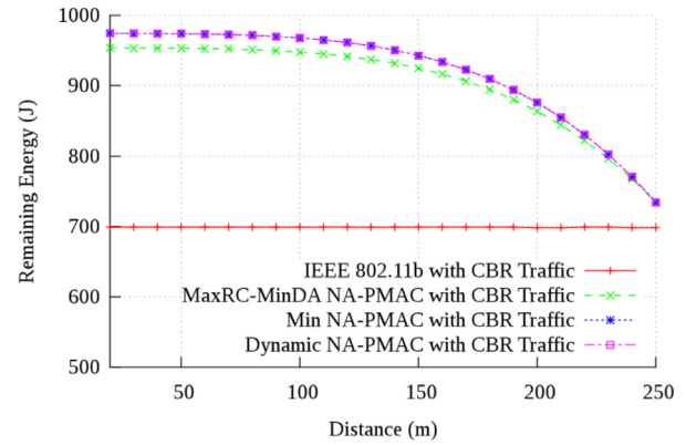
Fig. 6. Total remaining energy of the source.
