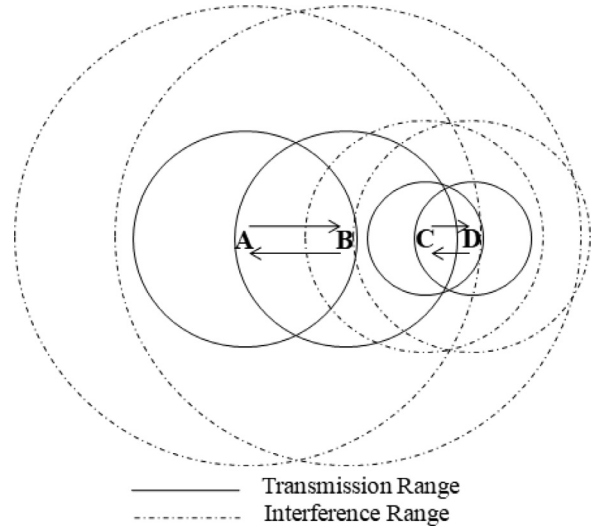
Fig. 4. Transmission power estimation without neighbour's power consideration.
