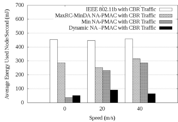
Fig. 18. Battery utilization in 500 m 2 with fewer source and destination pairs (i.e. three pairs).
