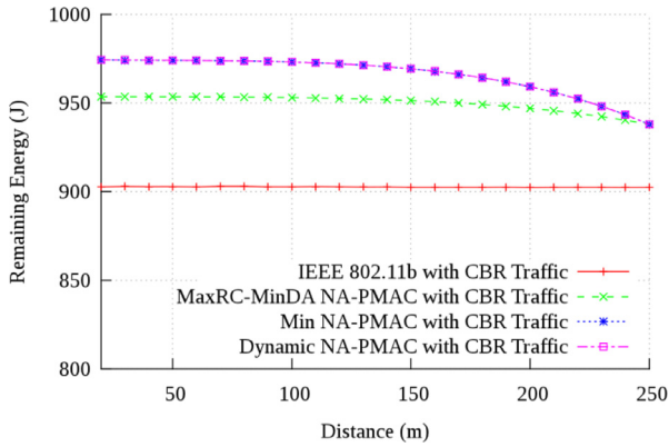
Fig. 7. Remaining energy at destination.
