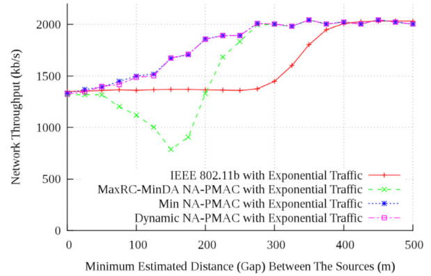
Fig. 12. Network performance of random sources and destinations using exponential traffic.
