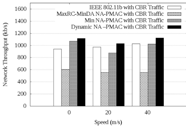
Fig. 17. Network performance in 500 m 2 with large source and destination pairs (i.e. ten pairs).
