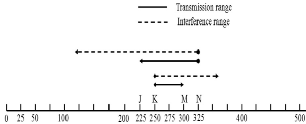
Fig. 8. Partial hidden node issue.
