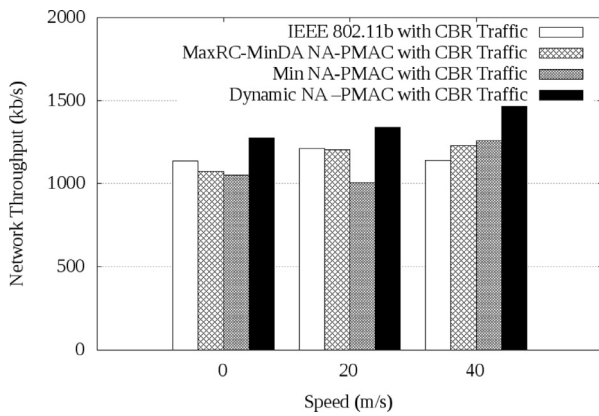
Fig. 16. Network performance in 500 m 2 with fewer source and destination pairs (i.e. three pairs).
