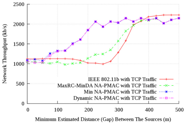
Fig. 13. Network performance of random sources and destinations using TCP traffic.
