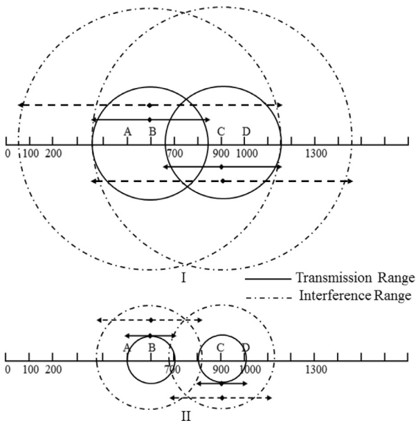
Fig. 1. (I) Sharing channel by using a fixed transmission Range (II) concurrency achieved by using an estimated power-controlled transmission.
