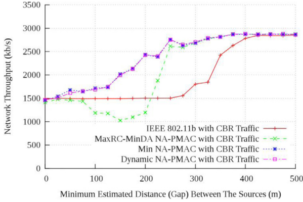
Fig. 11. Network performance of random sources and destinations using real time traffic (CBR).
