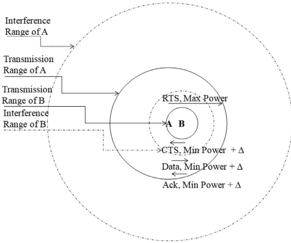
Fig. 3. Power adaptation when first RTS and CTS are exchanged.
