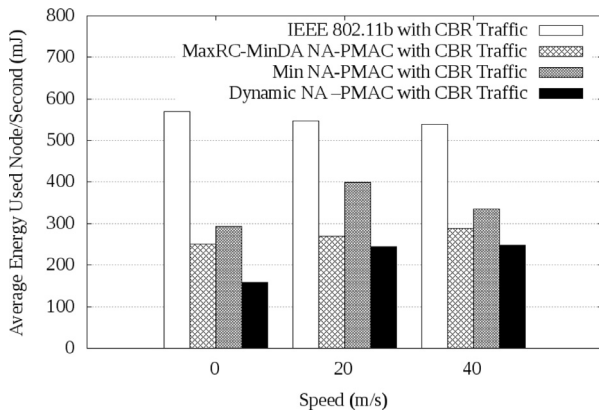
Fig. 23. Battery utilization in 1000 m 2 with large source and destination pairs (i.e. ten pairs).
