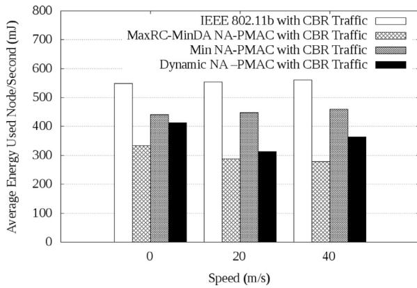
Fig. 22. Battery utilization in 1000 m 2 with fewer source and destination pairs (i.e. three pairs).
