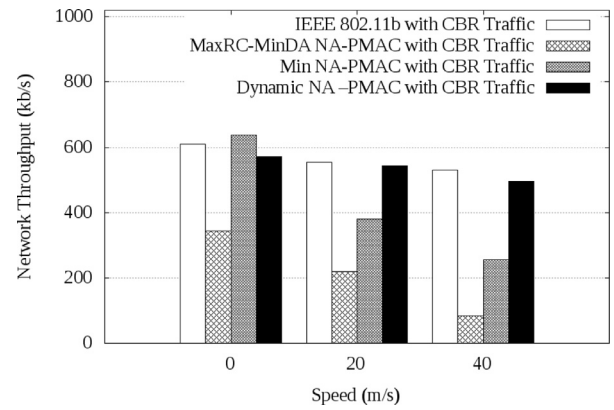
Fig. 20. Network performance in 1000 m 2 with fewer source and destination pairs (i.e. three pairs).
