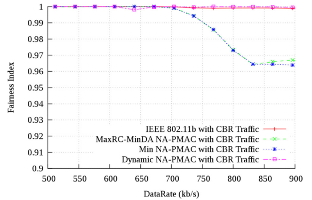
Fig. 9. Fairness index of partial hidden node issue.
