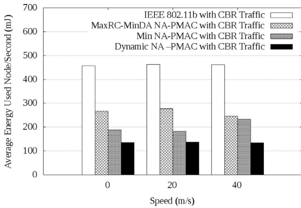
Fig. 19. Battery utilization in 500 m 2 with large source and destination pairs (i.e. ten pairs).
