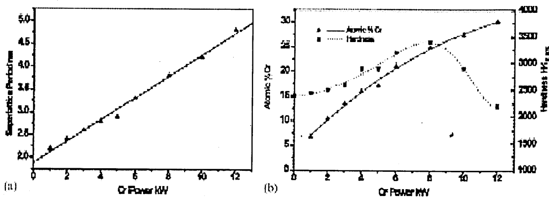
Figure 2-22: Cr power (Cr content) versus hardness and periodicity of the TiAlN/CrN nanolayers (superlattice period) [130].
