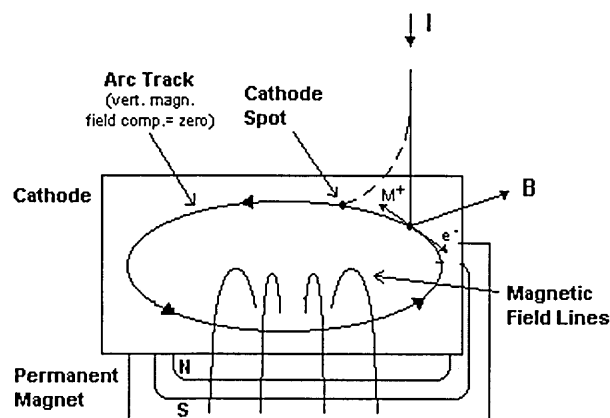
Figure 2-7: Arc spot motion in a steered cathodic arc
