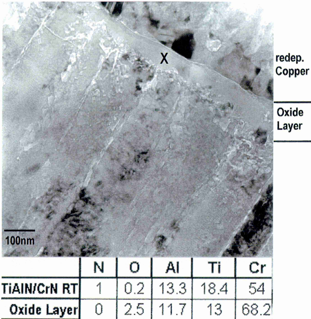
Figure 8-8: BF TEM image of the surface of TiAlN/CrN after heat treatment for 1h at 900°C, including results from EDX spot analysis performed using a probe of 40nm size in the TEM
