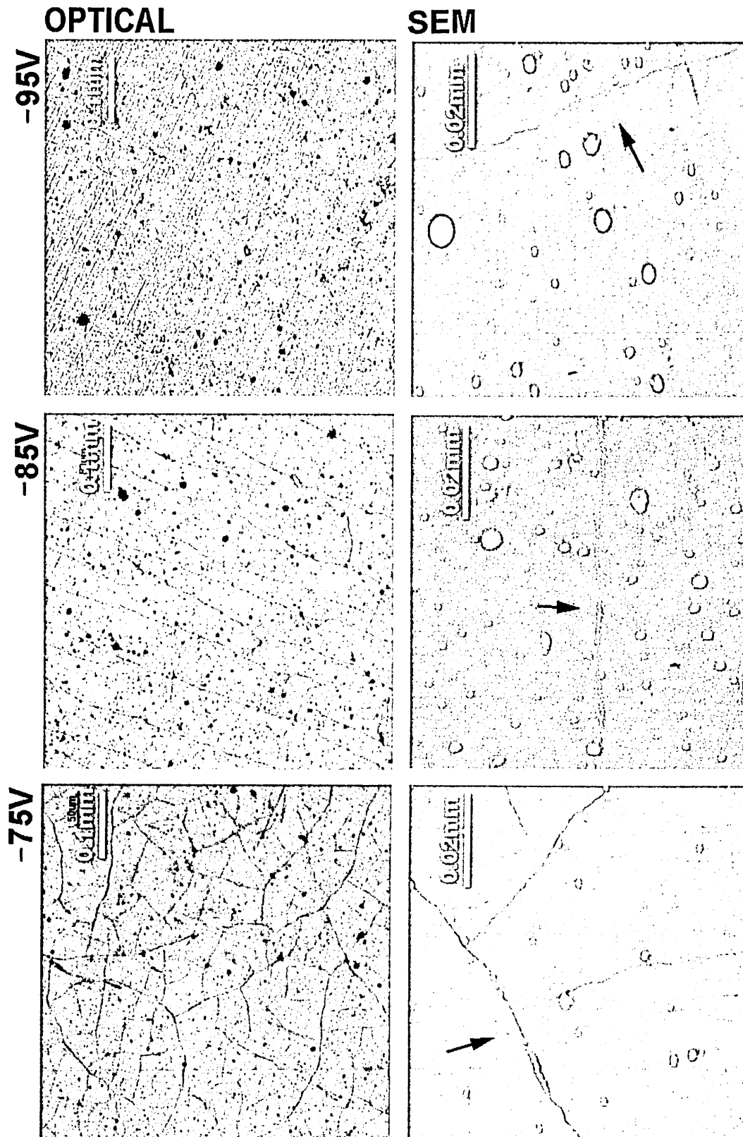
Figure 4-16: Cracks observed optically and using SEM on TiAlN/CrN deposited using different bias voltages after heat treatment for 1h at 900°C
