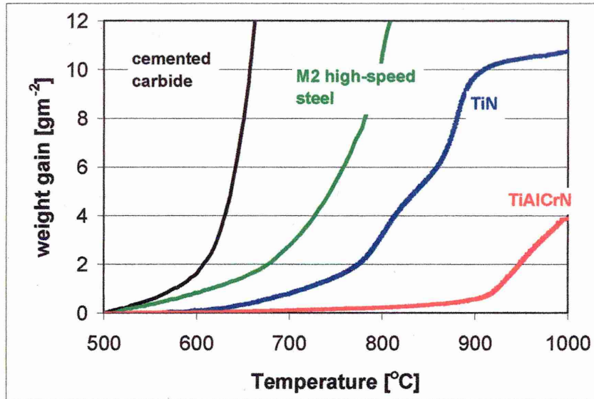
Figure 5-1: Continuous thermogravimetric measurement from Ti_{0.44}Al_{0.54}Cr_{0.02}N in comparison to tool materials.
