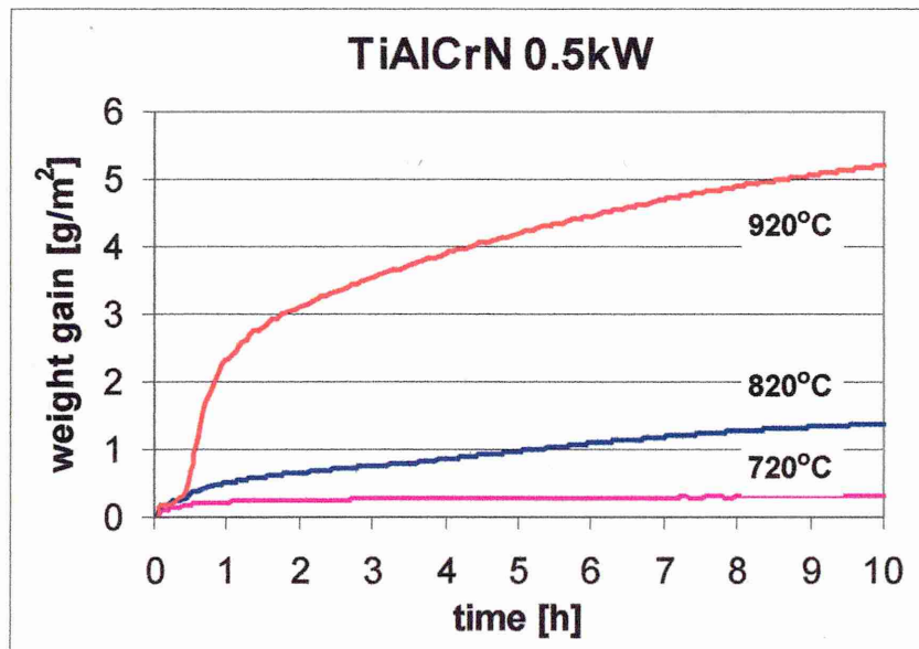
Figure 5-2: Isothermal thermogravimetric measurements of Ti_{0.44}Al_{0.54}Cr_{0.02}N .
