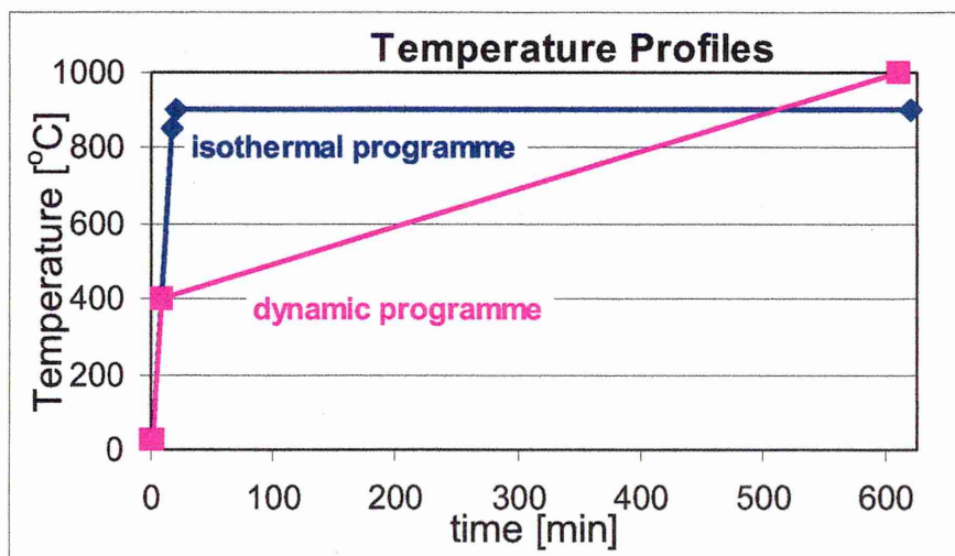
Figure 3-6: Temperature profiles of the TG programmes used
