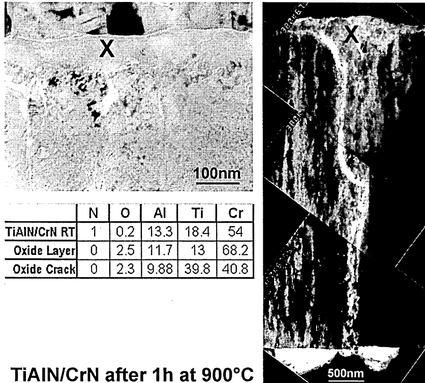
Fig.3: TEM bright field micrographs of TiAlN/CrN deposited at -75 V bias heat-treated for 1h at 900°C. The X indicate points where the EDX analysis was taken from. The analysis of the TiAlN/CrN coating was taken of the middle of the sample.
