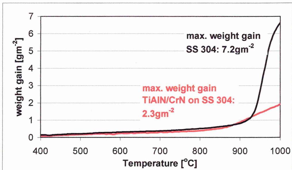
Figure 4-4: Continuous TG measurements on SS and \text{Ti}_{0.26}\text{Al}_{0.26}\text{N}/\text{Cr}_{0.48}\text{N}
