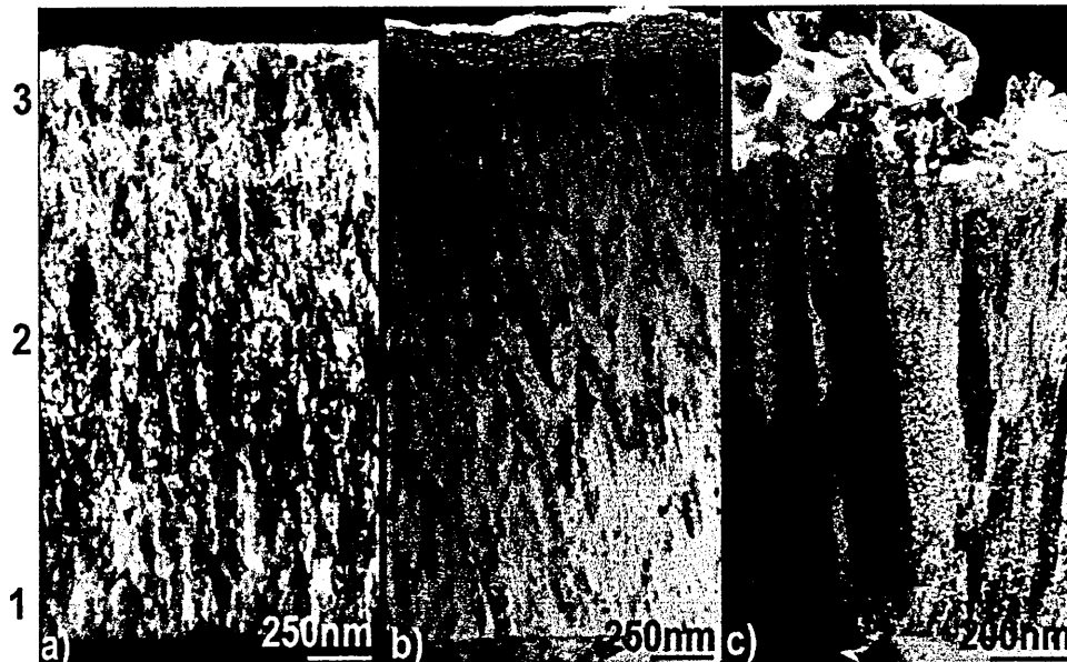
Figure 1. XTEM bright field images from TiAlCrYN with topcoat.
