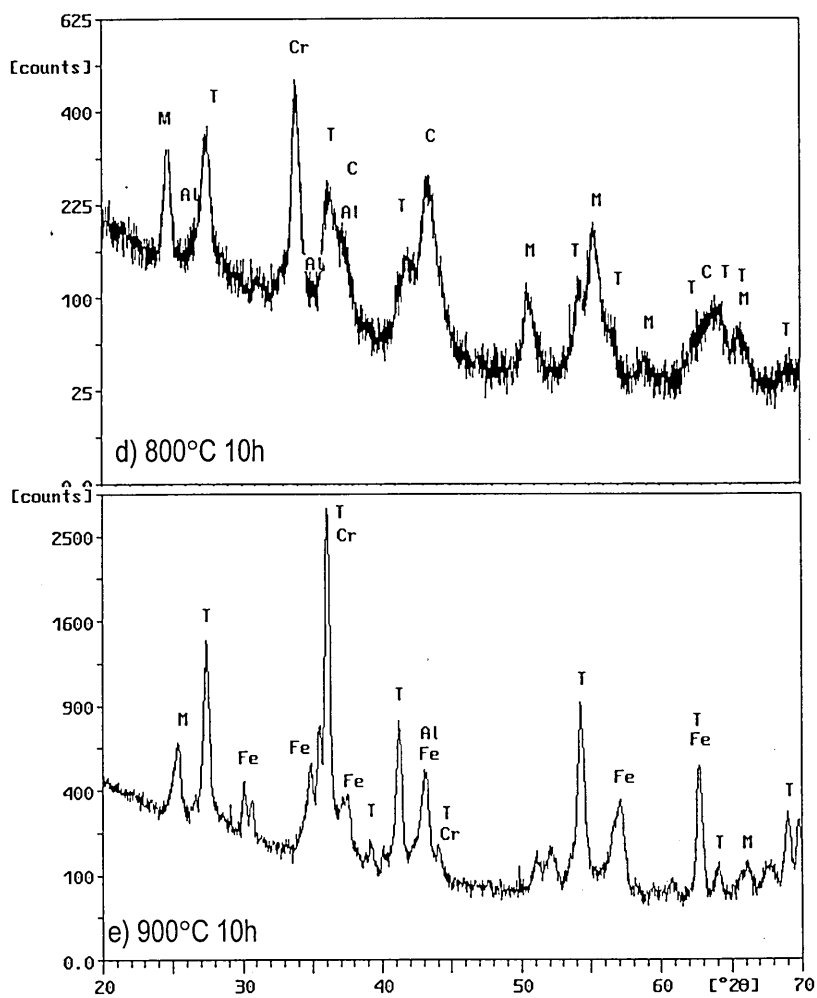
Figure 7-34: Glancing angle XRD at 0.5° incidence angle. TiAlCrYN+Ox at a) room temperature, b) after 600°C for 10h, c) after 700°C for 10h, d) after 800°C for 10h and e) after 900°C for 10h. The peak labels mean C=coating, T=TiO 2 (rutile), Al=Al 2 O 3 , Cr=Cr 2 O 3 , Fe=FeCr 2 O 4 and M=solid solution out of Al 2 O 3 and Cr 2 O 3 .
