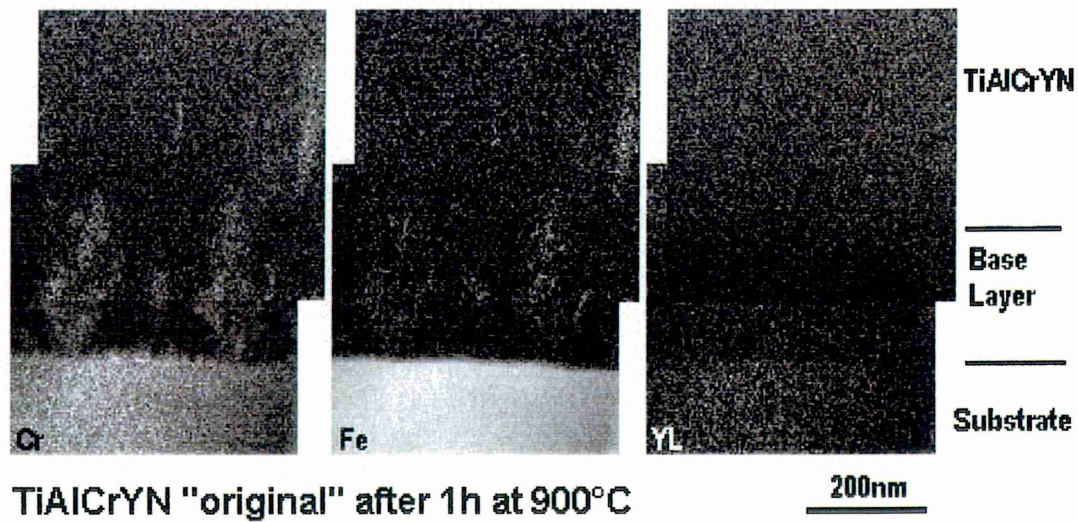
Figure 6-9: Cr, Fe and YL map from the base layer region of TiAlCrYN after heat treatment for 1h at 900°C.
