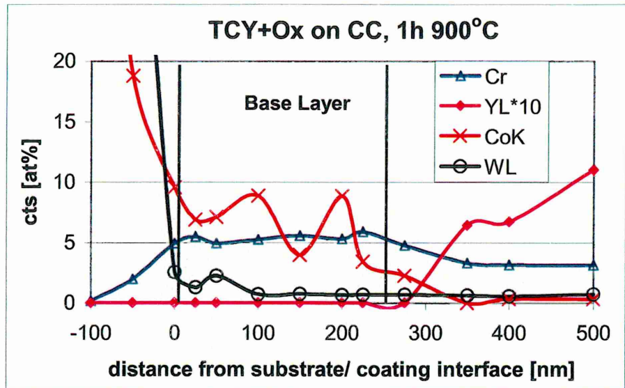
Figure 7-59: Point analysis profile in the base layer region of TiAlCrYN+Ox deposited onto stainless steel
