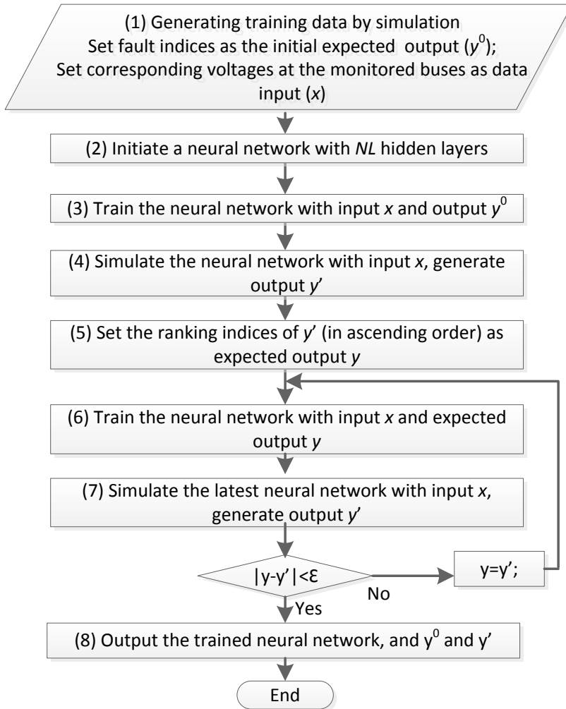
Fig. 3. Procedure of obtaining the neural network and corresponding representative fault indices.
