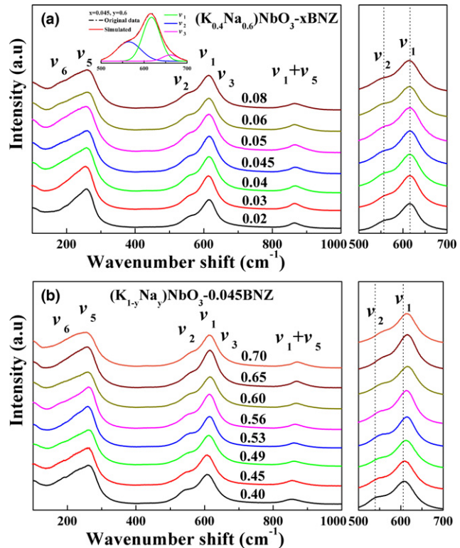
Fig. 3. Room temperature Raman spectra of KNyN-xBNZ (a) KN0.6N-xBNZ, inset shows the Raman amplified peaks around 600\text{ cm}^{-1} simulated by Gaussian and (b) KNyN-0.045BNZ.
