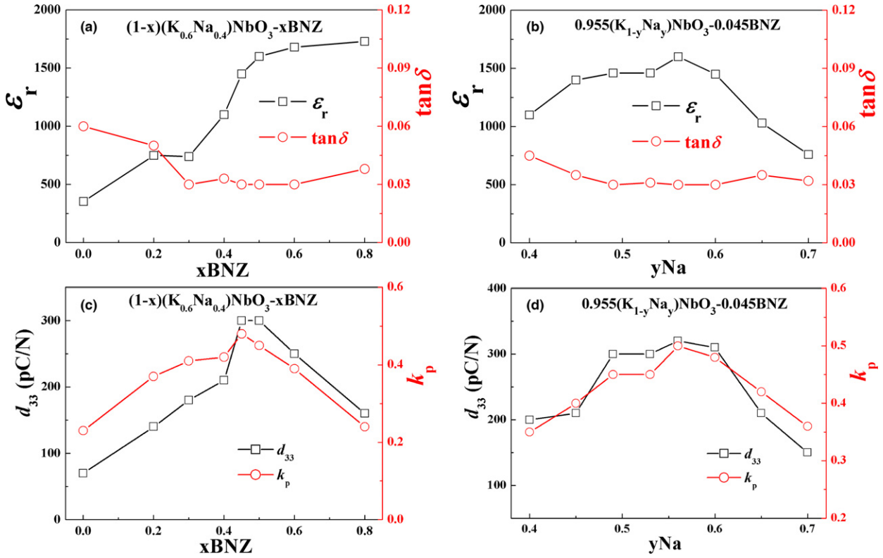
Fig. 6. Dielectric and piezoelectric properties of KNNy-xBNZ (a) \epsilon_r and \tan\delta as a function of BNZ, (b) \epsilon_r and \tan\delta as a function of Na, (c) d_{33} and k_p as a function of BNZ, (d) d_{33} and k_p as a function of Na.
