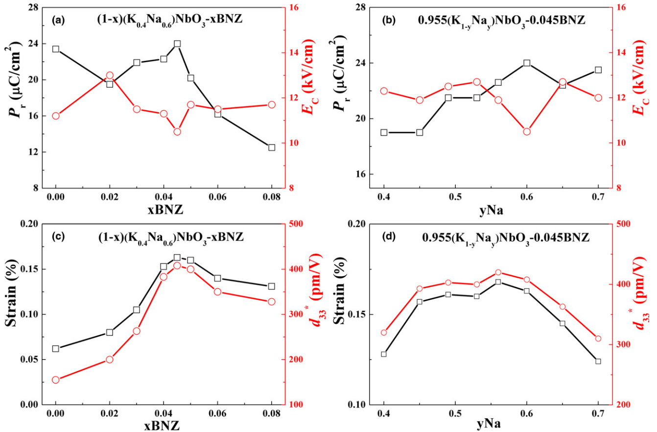
Fig. 5. Ferroelectric and strain properties of KNN-xBNZ (a) P_r and E_c as a function of BNZ, (b) P_r and E_c as a function of Na, (c) S and d_{33}^* as a function of BNZ, (d) S and d_{33}^* as a function of Na.
