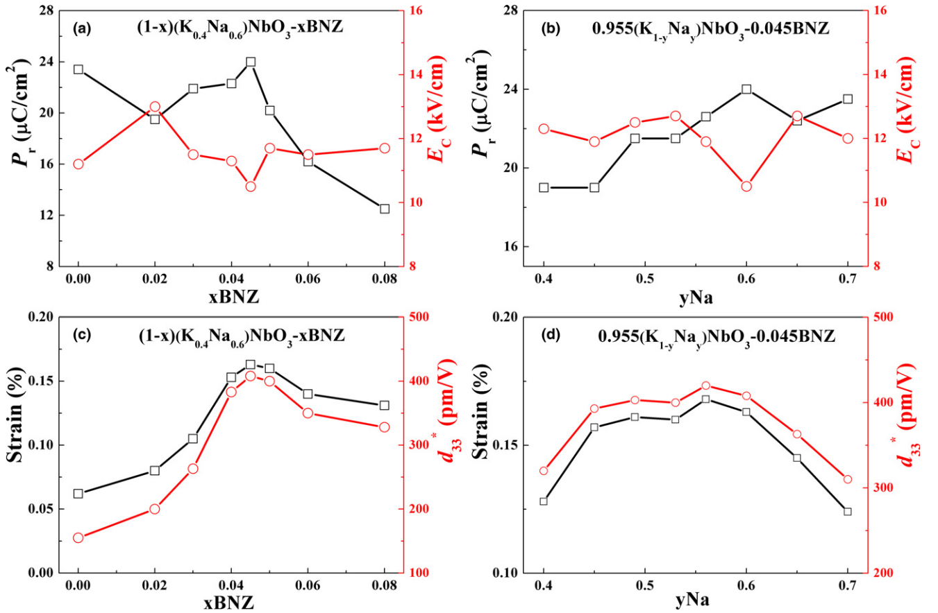
Fig. 5. Ferroelectric and strain properties of KNN- x BNZ (a) P_r and E_C as a function of BNZ, (b) P_r and E_C as a function of Na, (c) S and d_{33}^* as a function of BNZ, (d) S and d_{33}^* as a function of Na.
