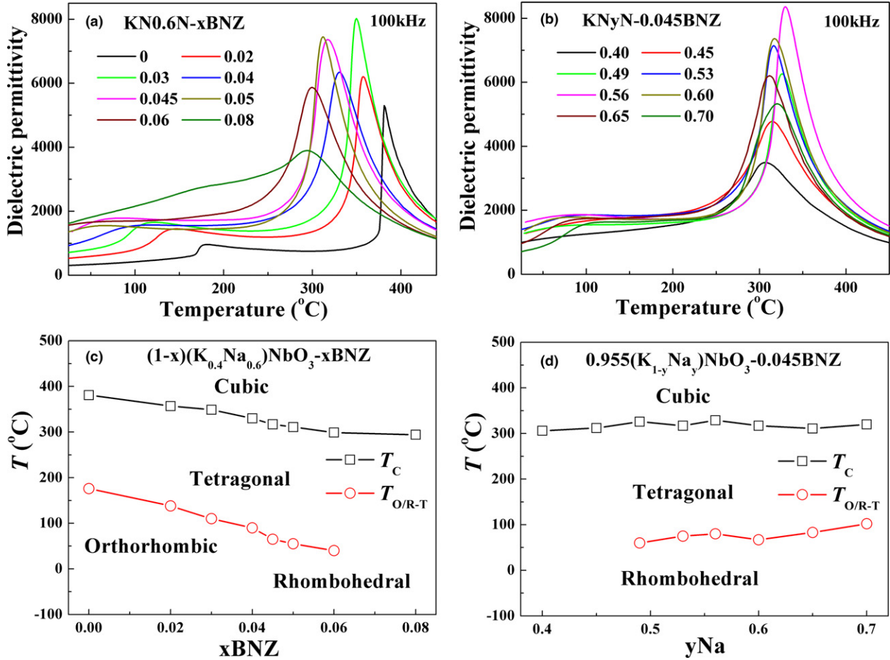
Fig. 7. Temperature dependence of \epsilon_r and \tan\delta for KNNy-xBNZ (a) KN0.6N-xBNZ, (b) KNNy-0.045BNZ, (c) T_C and T_{O/R-T} as a function of BNZ, (d) (c) T_C and T_{O/R-T} as a function of Na.
