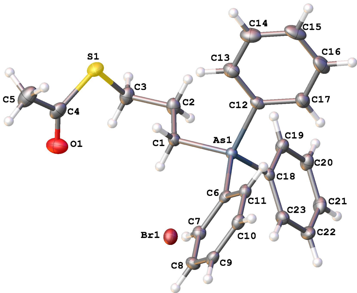
Fig. 2. Molecular structure of thioacetate salt 4.
