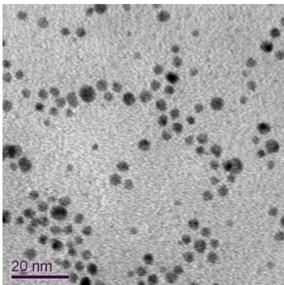
Fig. 4. TEM image of arsonium-AuNP derived from zwitterion 3 and associated particle size histogram.
