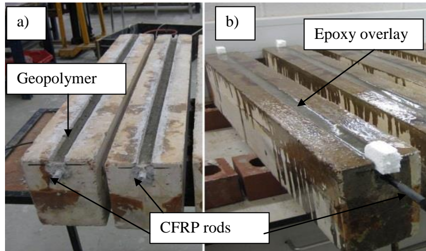
Figure 5. (a). Bonding CFRP rods to pre-grooved beams by geopolymer (first layer of repair material) (b). Overlay of epoxy as the second layer of repair
