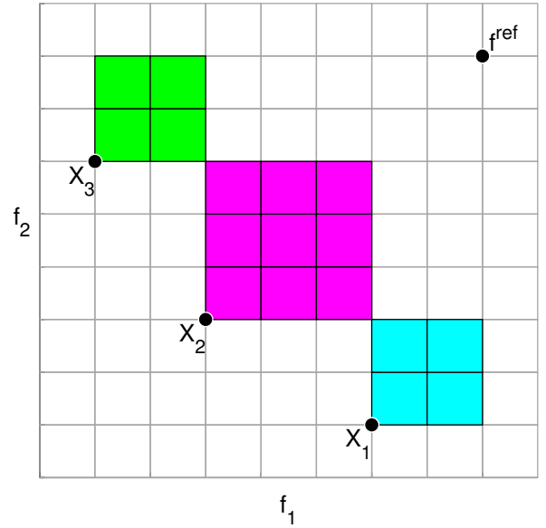
Figure 17: An example of the contributing hypervolume indicator in two-dimensional objective space.
