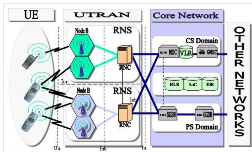
Fig. 2 UMTS Architecture
