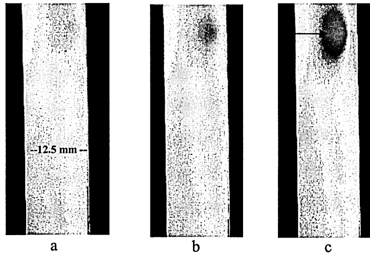
Figure IV.10. Thermographic images of fatigued Al/SiC p composite specimen showing the formation of plasticity zone before fracture occurs, (a) at 246500 cycles, (b) at 248600 cycles, and (c) at 251000 cycles, which corresponds to the specimen's fracture point.
