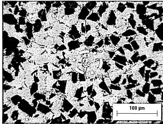
Figure III.7. Ingot A359/25 vol. % SiC p - Showing Dendritic Al-Si arms and homogeneous distribution of SiC p reinforcement.
