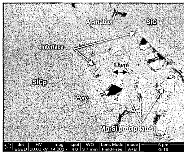
Figure III.12b. Hot rolled 31 vol. % SiC p – T6 showing Mg 2 Si precipitates formed between the SiC p reinforcement interface in a platelet shape of around 1-3 μm. A pore of similar size has been identified close to the interface.
