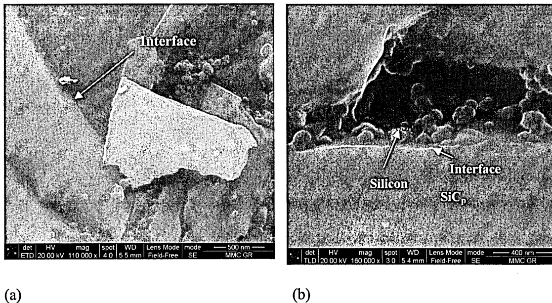
Figure III.9a. Hot Rolled A359/31 vol. % \text{SiC}_p showing Interface region. Figure III.9b.
