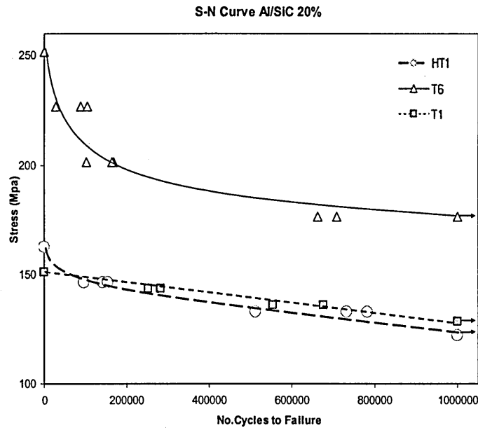
Figure IV.4a. S-N Curve of Al/SiC p 20 vol. % Composite
