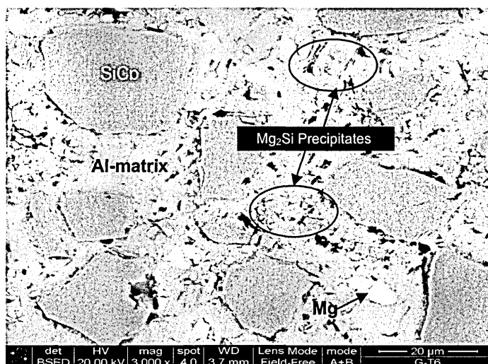
Figure III.12a. Hot rolled 31 vol. % \text{SiC}_p -T6 showing precipitates formed around the reinforcement.
