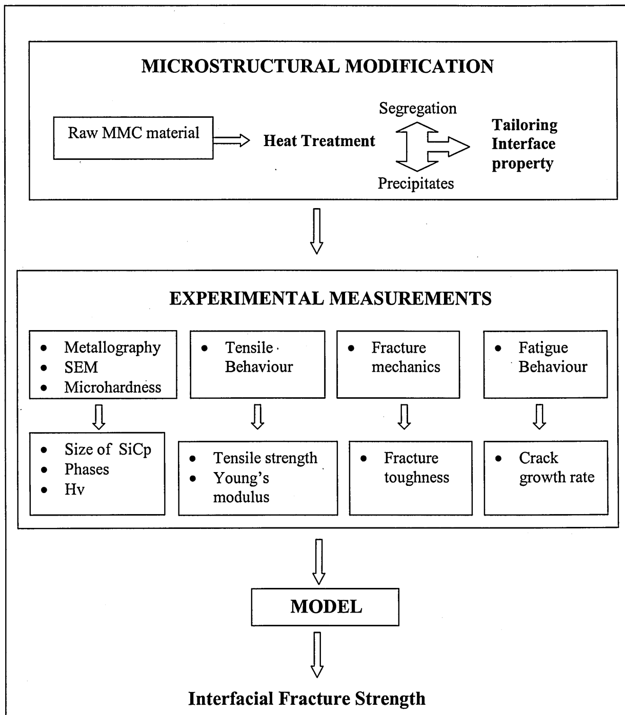
Figure I.1. The design of SiC particulate reinforced aluminium alloy composite system with tailored mechanical properties.
