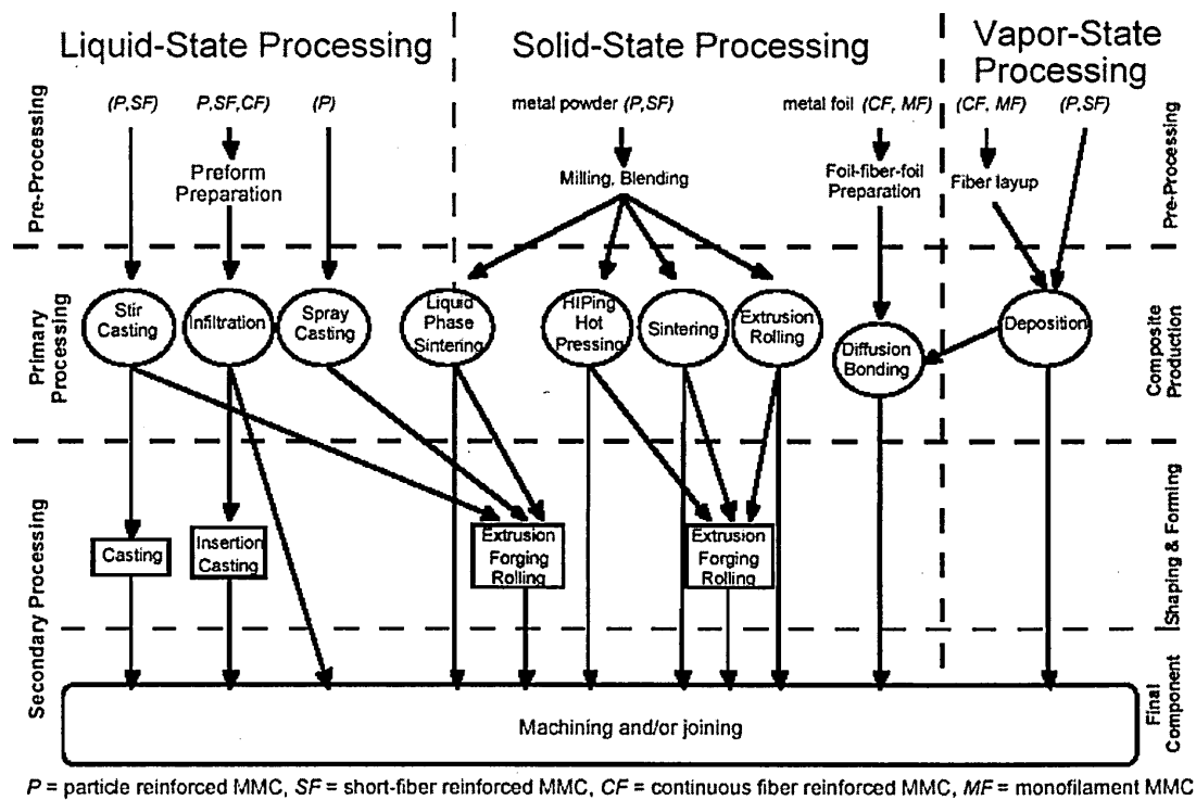
Figure II.2. Overview flow chart of MMC processing routes [35].
