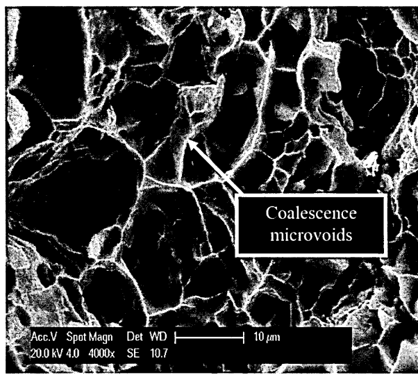
Figure IV.22c. T1 condition: Presence of coalescence microvoids indicating ductile behaviour.
