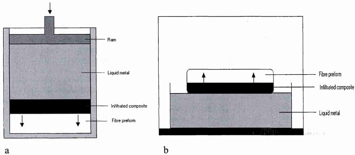
Figure II.3a, b. Infiltration process [36-37].
