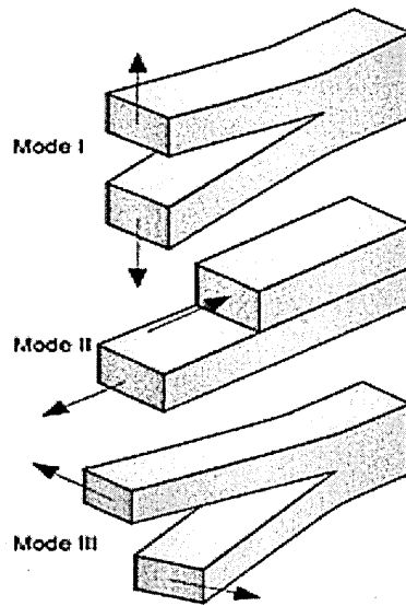
Figure II.7. The three modes of fracture [53].
