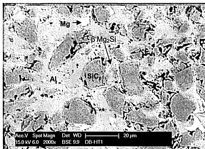
Figure III.10a. Microstructure of cast 30 vol. % \text{SiC}_p in the HT1 condition showing rod shape \beta' phases of \text{Mg}_2\text{Si} around the matrix and the interface of the reinforcement.
