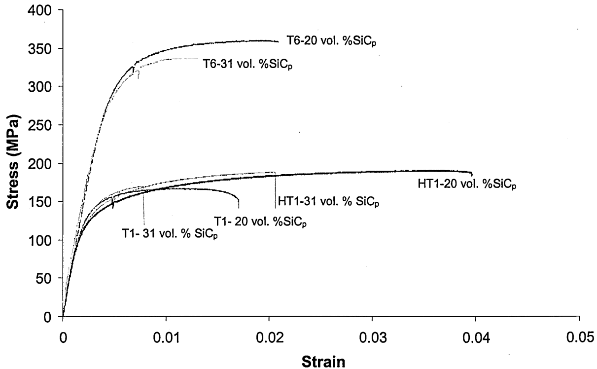
Figure IV.1. Average Stress / Strain curves of Al/SiC p Composites.
