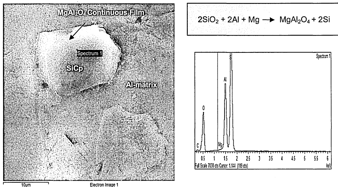
Figure III.15. \text{MgAl}_2\text{O}_4 phase observed to be a continuous film around the \text{SiC} particle. (white area)
