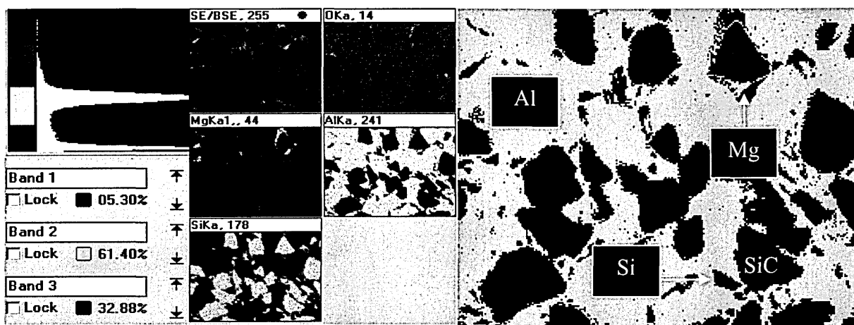
Figure III.4. SEM-Mapping Analysis of Cast A359/30 vol.% SiC p microstructure showing four distinct phases-Al, SiC p , Silicon and Magnesium
