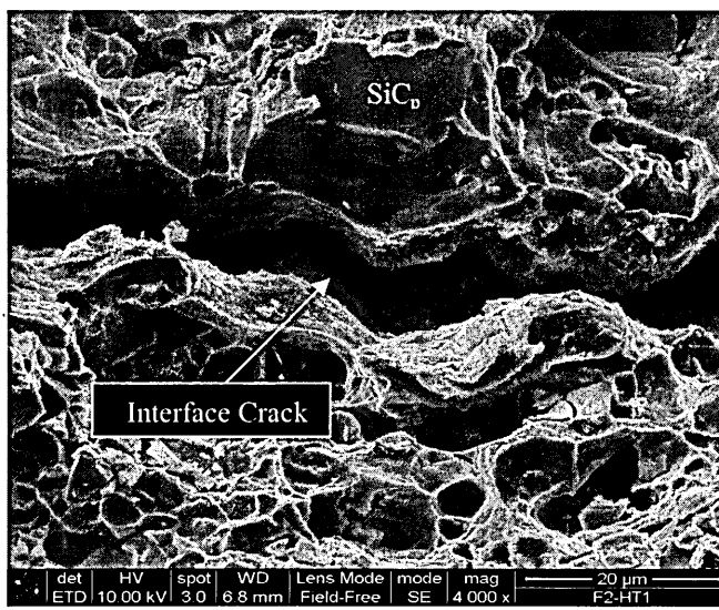
Figure IV.7a. Al/SiC p -HT1 condition- cracking through interface.
