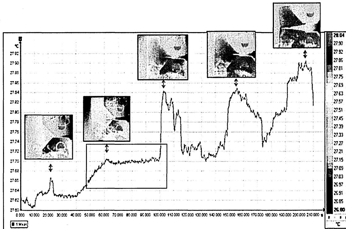
Figure IV.26c. Thermographic monitoring of Al/SiC p T6 composite CT specimen showing the different stages of crack growth up to the sample's final fracture.
