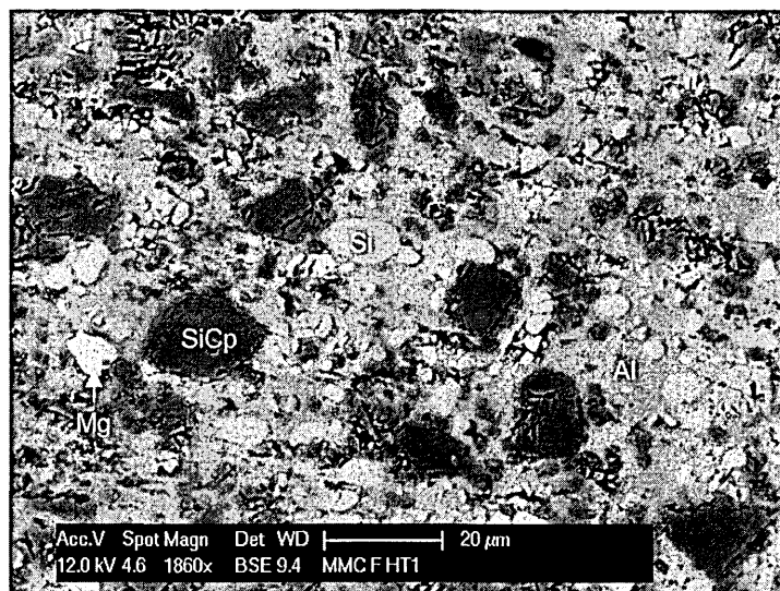
Figure III.11a Hot rolled 20 vol.% \text{SiC}_p HT1 sample showing phases of Aluminium, \text{SiC}_p , Silicon, Mg.
