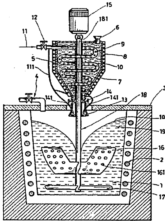
Figure II.6. Vortex method [44].
