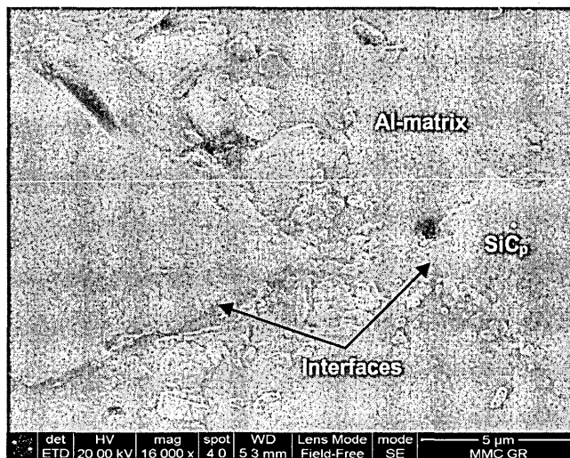
Figure III.8. Microstructure of rolled 31 vol. % SiC p in the T1 condition showing matrix-reinforcement interfaces.
