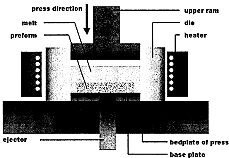
Figure II.5. Squeeze Casting [41].
