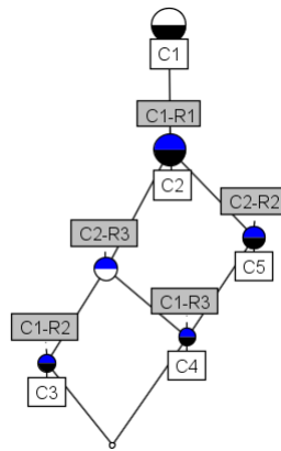
Fig. 6. The Corresponding Concept Lattice for the Simple Conceptual Graph
