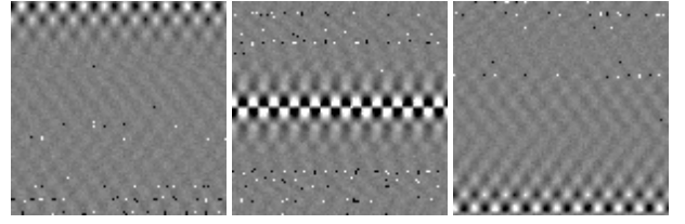
Figure 6: 1th, 50th and 99th image of a simulated focus set generated with povray [3]
