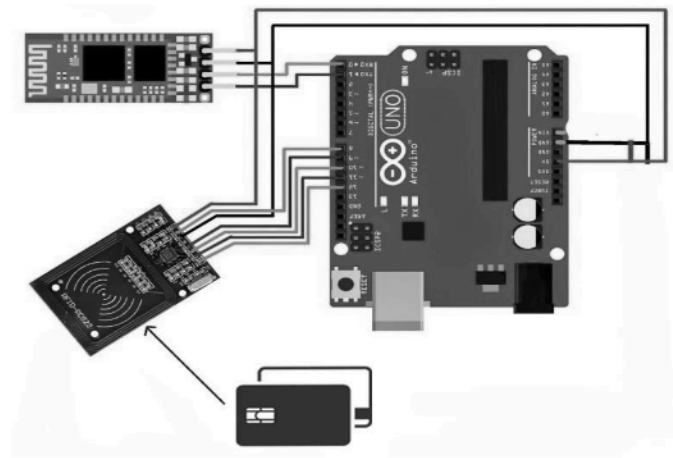
Fig. 2. IoT Based RFID tracking system Using Arduino Diagram
