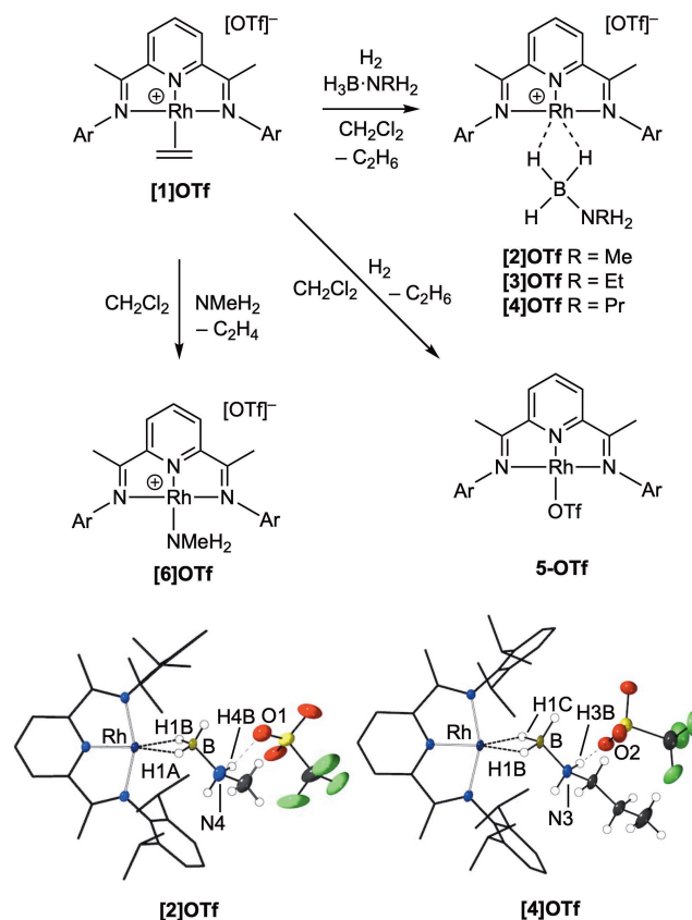
Scheme 2. Synthesis of complexes [\text{Rh}(\text{L1})(\text{ligand})][\text{OTf}] and molecular structures of [2]OTf and [4]OTf . \text{Ar} = 3,5- \text{Pr}_2\text{C}_6\text{H}_3 . Selected structural metrics ( \text{\AA} ): [2]OTf \text{Rh}\cdots\text{B} , 2.253(4); \text{B}\cdots\text{N4} , 1.581(7); \text{Rh}\cdots\text{H1A} , 1.89(3); \text{Rh}\cdots\text{H1B} , 1.88(3); \text{H4B}\cdots\text{O1} , 1.986(4). [4]OTf (one of two independent cations in the unit cell) \text{Rh}\cdots\text{B} , 2.290(4); \text{B}\cdots\text{N3} , 1.584(5); \text{Rh}\cdots\text{H1B} , 1.90(5) \text{\AA} ; \text{Rh}\cdots\text{H1C} , 1.89(4); \text{H3B}\cdots\text{O2} , 2.053(3).
