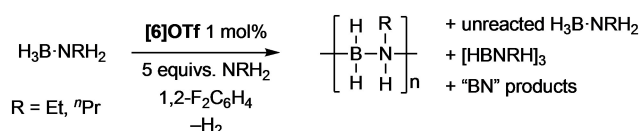
Scheme 7. Unselective dehydropolymerization of \text{H}_3\text{B-NR}'\text{H}_2 ( \text{R} = \text{Et}, ^n\text{Pr} ).
