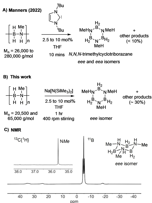
Scheme 5. A) Manners' report of depolymerization of [\text{H}_2\text{BNMeH}]_n using t -Bu ( i -Bu = 1,3-di- tert -butylimidazol-2-ylidene). B) Depolymerization using \text{Na}[\text{N}(\text{SiMe}_3)_2] . C) ^{11}\text{B} and ^{13}\text{C}\{^1\text{H}\} NMR spectrum of reaction mixture after 1 h showing the selective formation of the eee -isomer of [\text{H}_2\text{BNMeH}]_3 using polymer produced from [6]OTf , and 10 mol% \text{Na}[\text{N}(\text{SiMe}_3)_2] .
