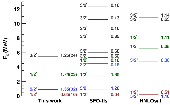
Fig. 6. Experimental level scheme for ^{15}\text{C} compared to the results of the shell model with the SFO-tls interaction and to SCGF calculations using the NNLO sat interaction. The column on the right represents the spectroscopic factor and on the left the spin and parity assignment.
