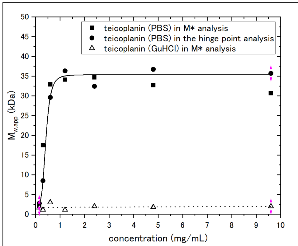
Figure 4. Change of weight average molar mass M_w of teicoplanin with loading concentration derived from sedimentation equilibrium analysed by SEDFIT-MSTAR 40 . Solid square symbols are molar masses M_{w,app} obtained from the M^* method. Solid round symbols are molar masses M_{w,app} obtained from the hinge point method. Solid line is a standard French curve fit to the data. Open triangle symbols are molar masses M_{w,app} of teicoplanin dissolved in 6M GuHCl from the M^* method.
