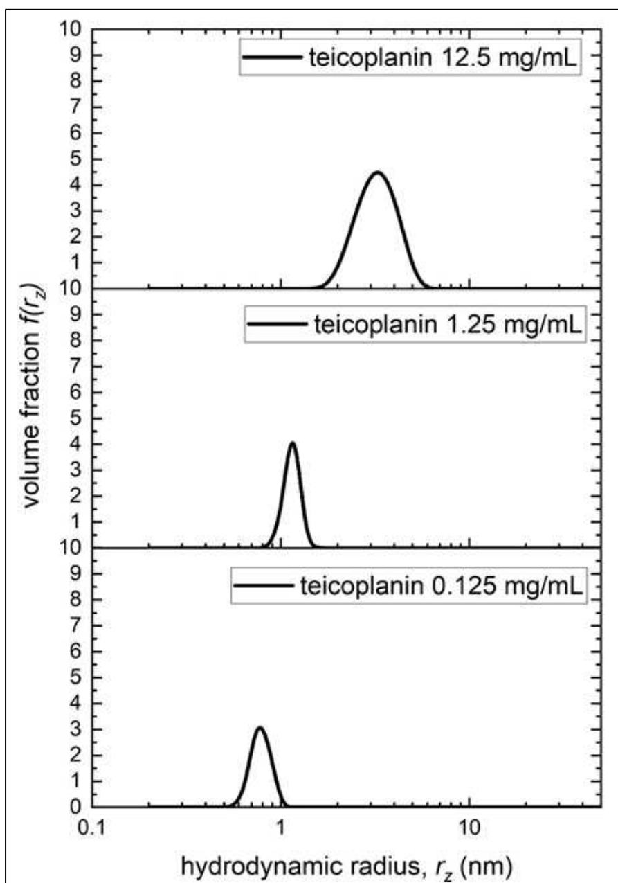
Figure 5. Distribution of z-average hydrodynamic radii obtained from dynamic light scattering measurements at 20.0°C for teicoplanin in solution at concentrations 12.5, 1.25 and 0.125 mg/mL
