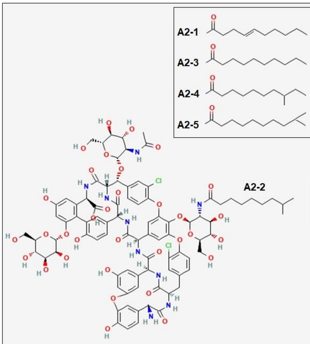
Figure 1. Structure of teicoplanin (adapted from the National Institute for Health/ National Center of Biotechnology Information 32 based on an original structure given by F. Parenti 33 ). Teicoplanin lipoform A2-2 ( M_1 = 1879.7 \text{ g/mol} ) is shown: the other major lipoforms of A2 with different acyl chains are shown in the inset
