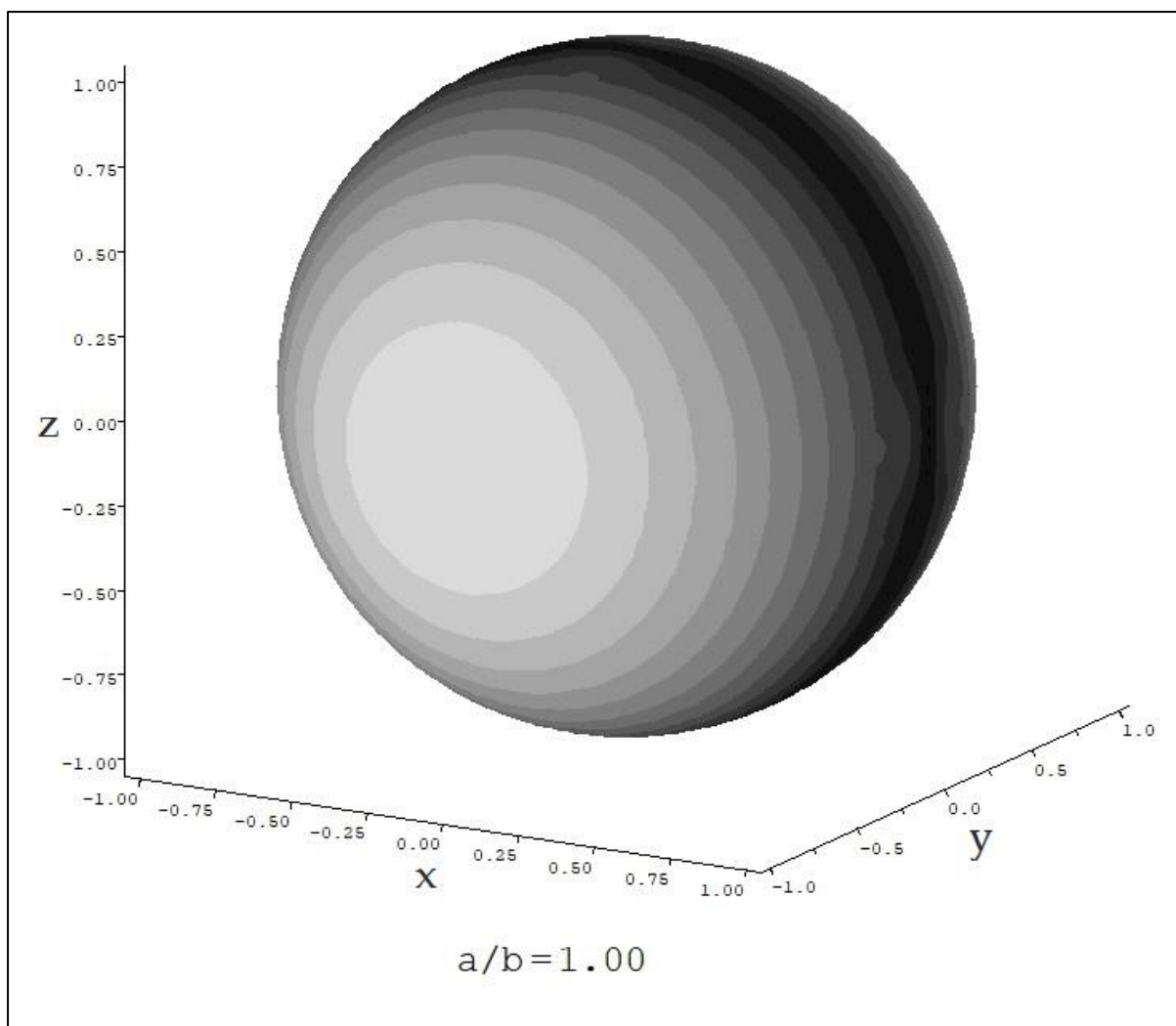
Figure 6. ELLIPS1 49 representation of the conformation of teicoplanin showing an axial ratio ( a/b ) = 1: i.e. a sphere
