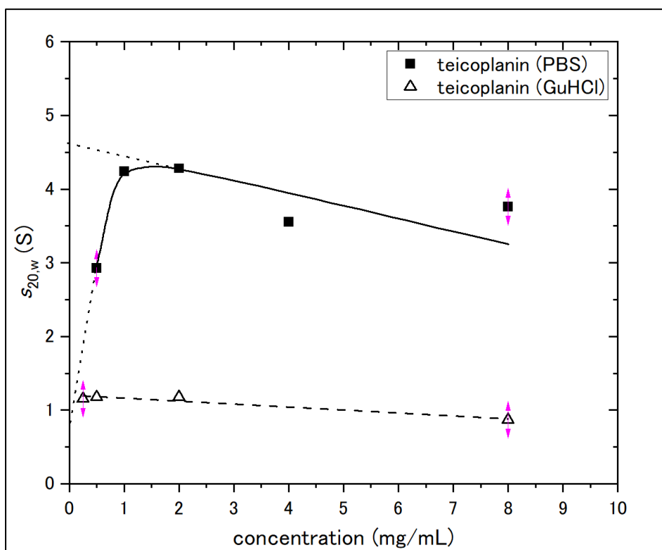
Figure 3. Change of apparent sedimentation coefficient ( s_{20,w} ) of teicoplanin A2 with sedimenting concentration, c . Concentrations were corrected for radial dilution. The extrapolated value of \sim 4.65 S is consistent with a spherical 18-19-mer of the molar mass of 35400. The lower extrapolated value of \sim 0.7 S is the predicted value for a spheroidal unimer, which is consistent with the s -value of teicoplanin dissolved in 6M GuHCl, s_{20,w} = (1.17 \pm 0.01) S. Solid line is a standard French curve fit to the data.
