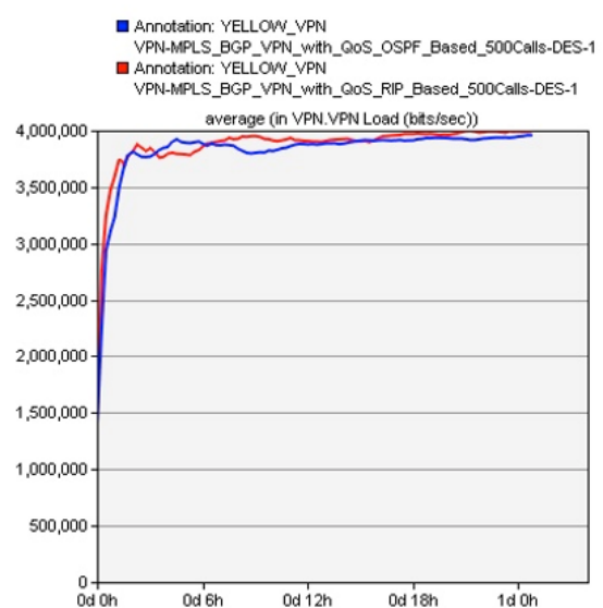
Figure 7. MPLS-VPN load
