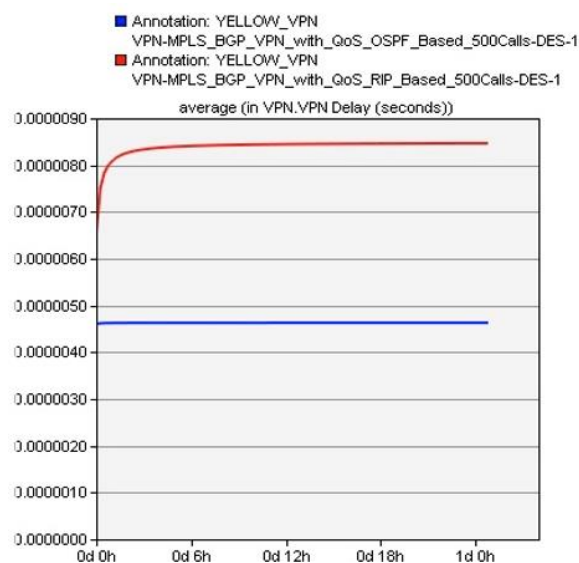
Figure 6. MPLS-VPN delay
