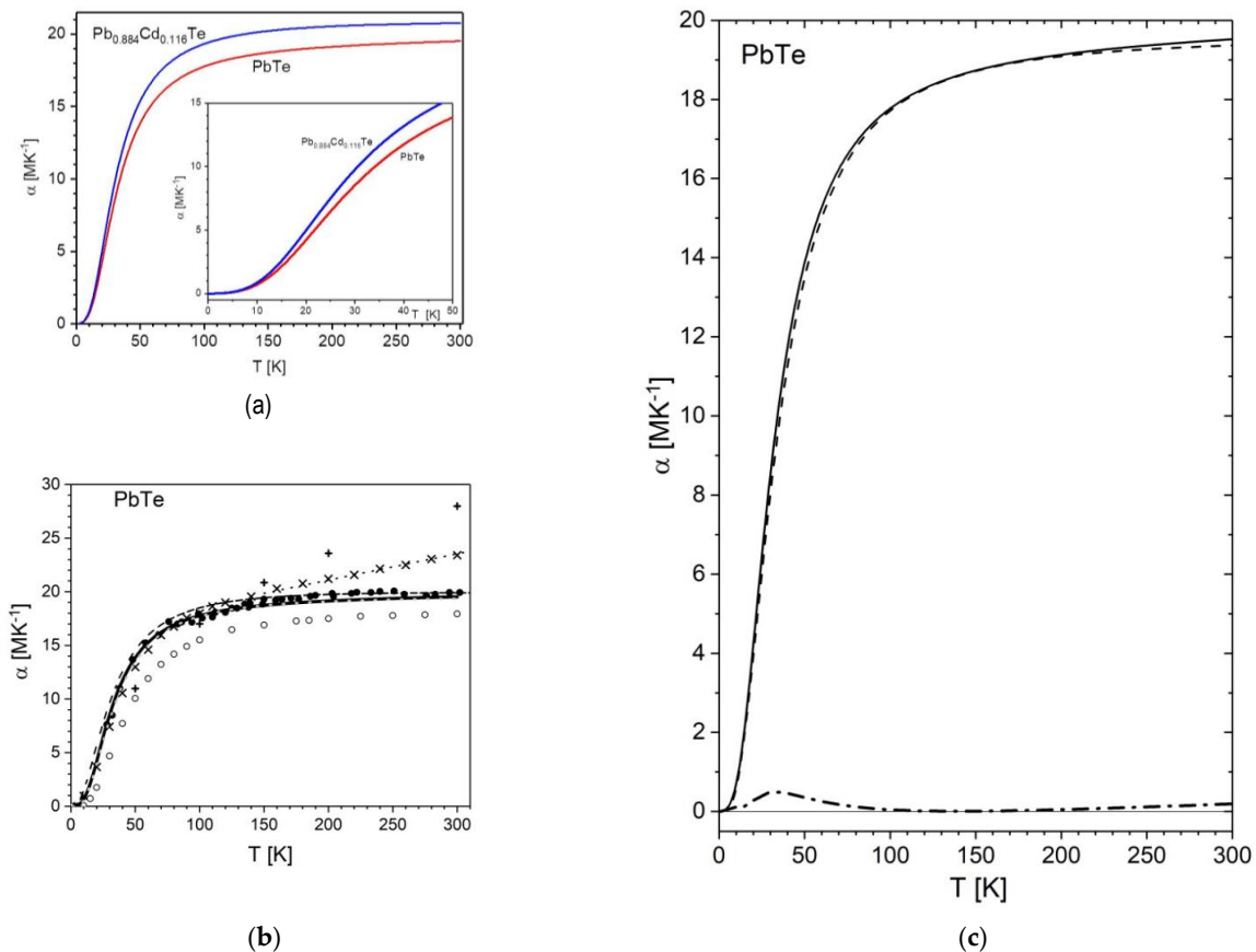
Figure 3. Variation of thermal expansion with temperature, \alpha(T) . (a) The linear thermal expansion coefficient \alpha(T) for \text{PbTe} and \text{Pb}_{0.884}\text{Cd}_{0.116}\text{Te} as a function of temperature, was obtained from the experimental-data fitting using a second order Grüneisen approximation (Equation (1)). The inset includes the magnified low-temperature part (0–50 K) of the \alpha(T) run. (b) Comparison of the present data for \text{PbTe} (black solid line) with previously reported experimental and theoretical data of \text{PbTe} . Selected data from literature (from ref. [51] (●), [29] (black dashed line) (experimental), (from ref. [45] (+); [46] (×), from ref. [8] (⊙) (theoretical)) are shown. (c) Comparison of the present experimental data (solid line, also shown as (strongly overlapping) dotted line in (b)), theory [60,108] (dashed line), difference curve (dash-dot line).
