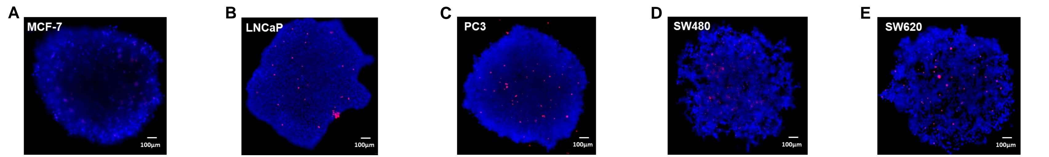
Figure 3. Human breast, prostate and colorectal cancer cell lines form viable and intact spheroids. Single spheroids generated by hanging drop were harvested at day 3 for viability assessment using Hoechst 33342/PI staining. MCF-7 (A), LNCaP (B), PC3 (C), SW480 (D) and SW620 (E) cancer cells form viable and intact spheroids at day 3 in hanging drop. MDA-MB-231 cancer cells disaggregate upon harvesting from the petri dish lid. Day 3 viability for MDA-MB-231 cancer cells was assessed by flow cytometry. Scale bar represents 100 µm.
