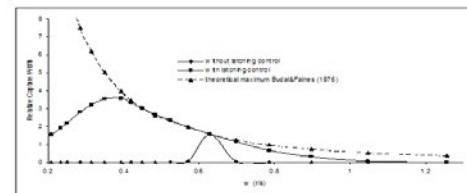
Figure 10: Relative capture width with and without latching control for a vertical-cylinder wave energy converter in the range of frequencies with 1m wave amplitude
