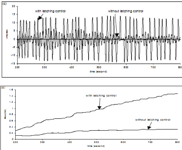
Figure 13: Comparison of different variables with and without latching control at natural period T_n=10s and peak period T_p=10s of vertical-cylinder wave energy converter (a) incident wave elevation at the origin of the wave energy converter (b) heave motion amplitude (c) heave velocity (d) accumulation of instantaneous absorbed power
