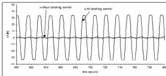
Figure 4: Heave motion amplitude of a vertical-cylinder wave energy converter with and without latching control at resonance period of 10s and incident wave period at 15s with 1m wave amplitude. In Figure 4, the numerical simulation in the time domain of the
