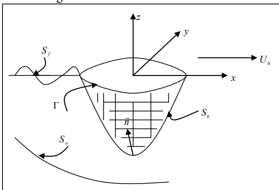
Figure 1: Coordinate system and surface of the problem
