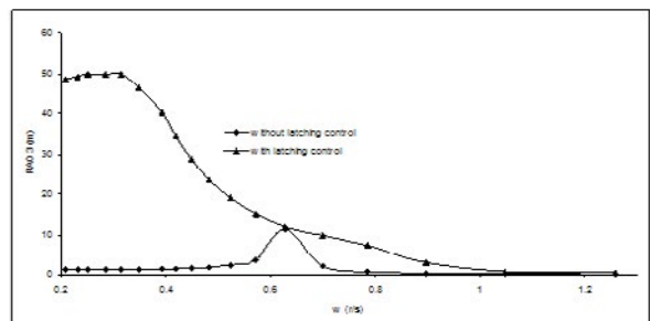
Figure 7: Heave Response Amplitude Operator (RAO) with and without latching control for a vertical-cylinder with 10s natural period and 1m wave amplitude for different range of frequencies. It is assumed that the excitation force is known in the future of the
