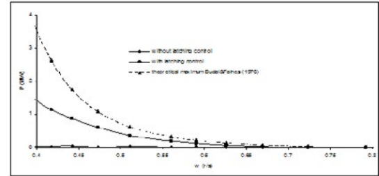
Figure 16: Absorbed mean power for a vertical-cylinder with and without latching control in the range of peak frequencies.
