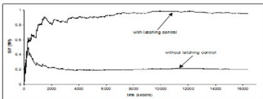
Figure 15: Convergence of mean power with and without latching control at natural period T_n = 10s and peak period T_p = 10s of vertical-cylinder wave energy converter
