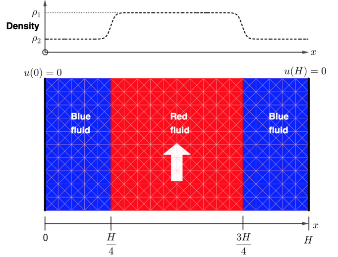
FIG. 9. Schematic representation of the geometry and transverse density stratification used in the pressure gradient (white arrow) driven flow tests.
