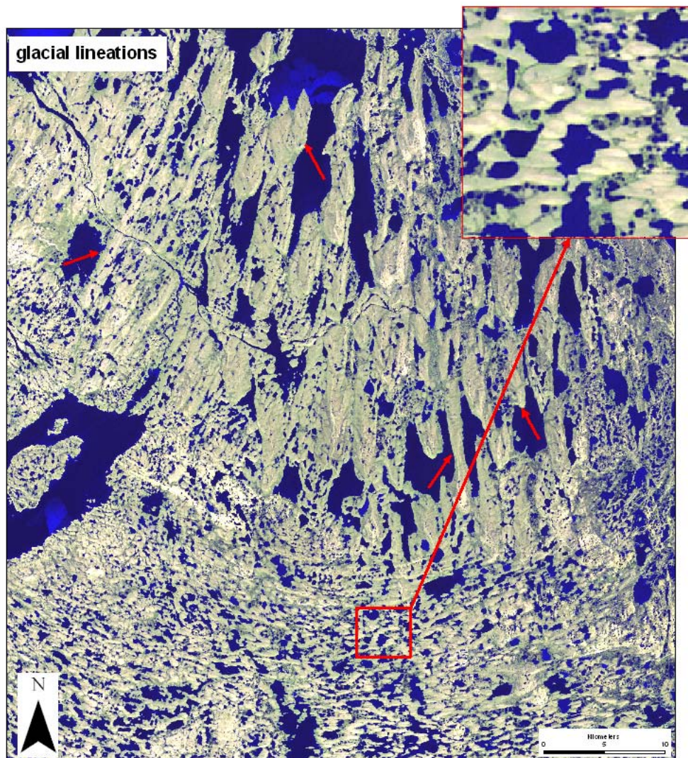
Figure 2 Landsat ETM+ satellite image (R,G,B: 7,5,2) of glacial lineations in south-eastern Victoria Island. The top half of the image shows large mega-scale glacial lineations (MSGSL) indicating flow from south to north (individual landforms highlighted with red arrows). The bottom half of the image shows smaller glacial lineations (drumlins) superimposed on the MSGSL and indicating a younger ice flow from east to west (see inset). See Figure 1 for location.
