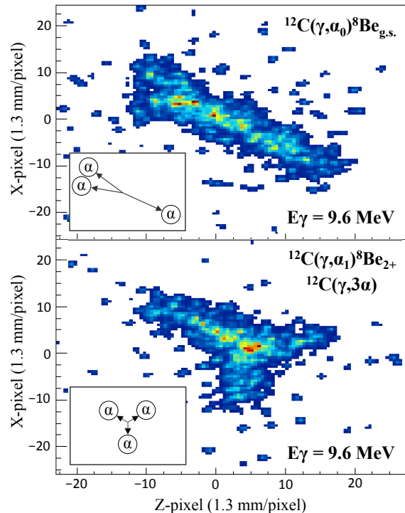
FIG. 1. (Color online) Different types of events photographed by the O-TPC for E_\gamma = 9.6 MeV. Upper panel: A {}^{12}\text{C}(\gamma, \alpha_0){}^8\text{Be}_{\text{g.s.}} sequential decay. Lower panel: A {}^{12}\text{C}(\gamma, \alpha_1){}^8\text{Be}_{2^+} sequential decay or {}^{12}\text{C}(\gamma, 3\alpha) direct decay, which are indistinguishable.
