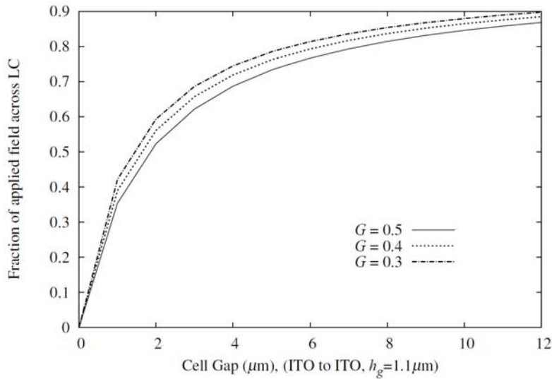
Figure 8. Approximation for the electric field across a grating aligned LCD. a) Definition of FWHM = X and pitch = X+Y ; b) equivalent circuit for grating; c) E field across LC as a function of cell gap and shape factor G = \text{FWHM} / \text{Pitch} (=X/X+Y) .
