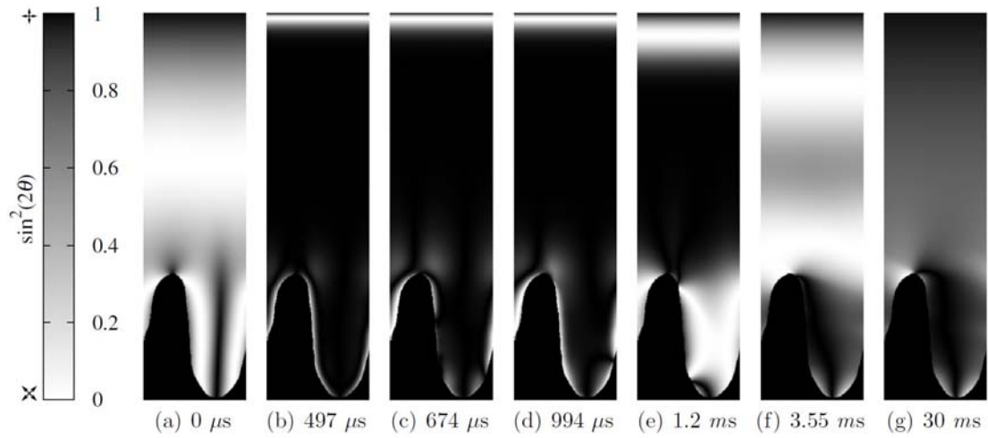
Figure 2. Typical representation of C to D latching dynamics in a ZBD cell at a voltage 1 volt above the latching threshold and \tau = 500 \mu\text{s} , where t = 0 corresponds to the initial application of the bi-polar pulse, t = 500 \mu\text{s} corresponds to the reversal of the field half way through the bipolar pulse and the electric field is removed at t = 1 \text{ms} . Shown is the director polar angle only; there is also a \sim \pi/4 twist in the equilibrium states from parallel to the plane of the paper at the lower grating surface, to perpendicular to the plane of the paper at the upper flat surface.
